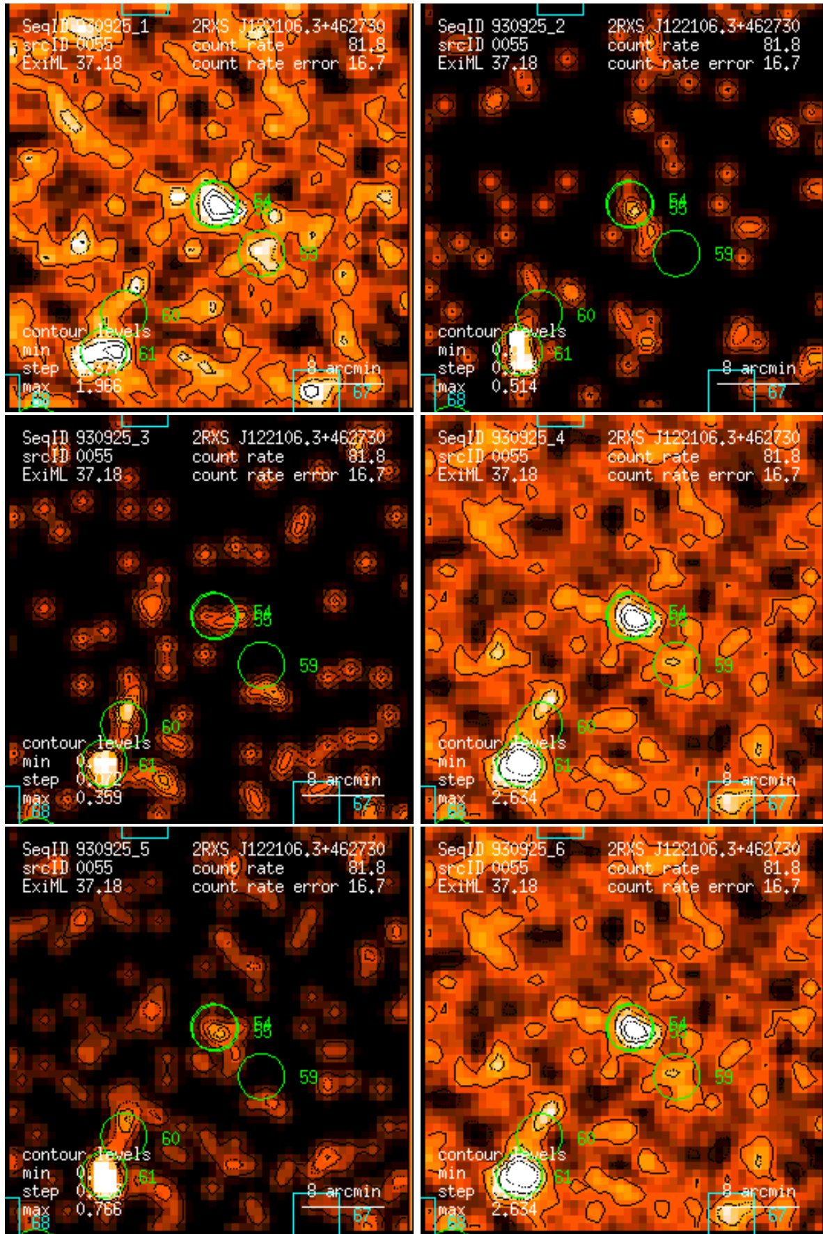
Figure 55: RASS 930925: detection 0055: band rate images, Gaussian filter: (1) PSPC channels 11 – 41, (2) 52 – 90, (3) 91 – 201, (4) 11 – 235, (5) 52 – 201, (6) 11 – 201. Broad band rates in counts/ks. Band rate contour levels in counts/ks/arcmin 2 .
