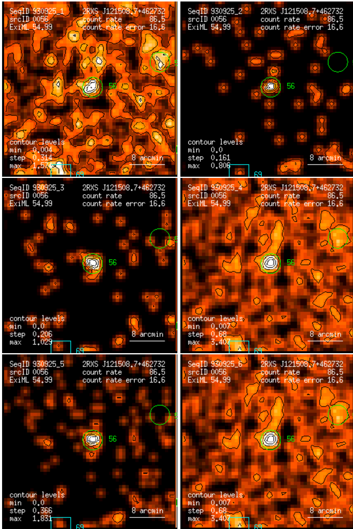
Figure 56: RASS 930925: detection 0056: band rate images, Gaussian filter: (1) PSPC channels 11 – 41, (2) 52 – 90, (3) 91 – 201, (4) 11 – 235, (5) 52 – 201, (6) 11 – 201. Broad band rates in counts/ks. Band rate contour levels in counts/ks/arcmin 2 .
