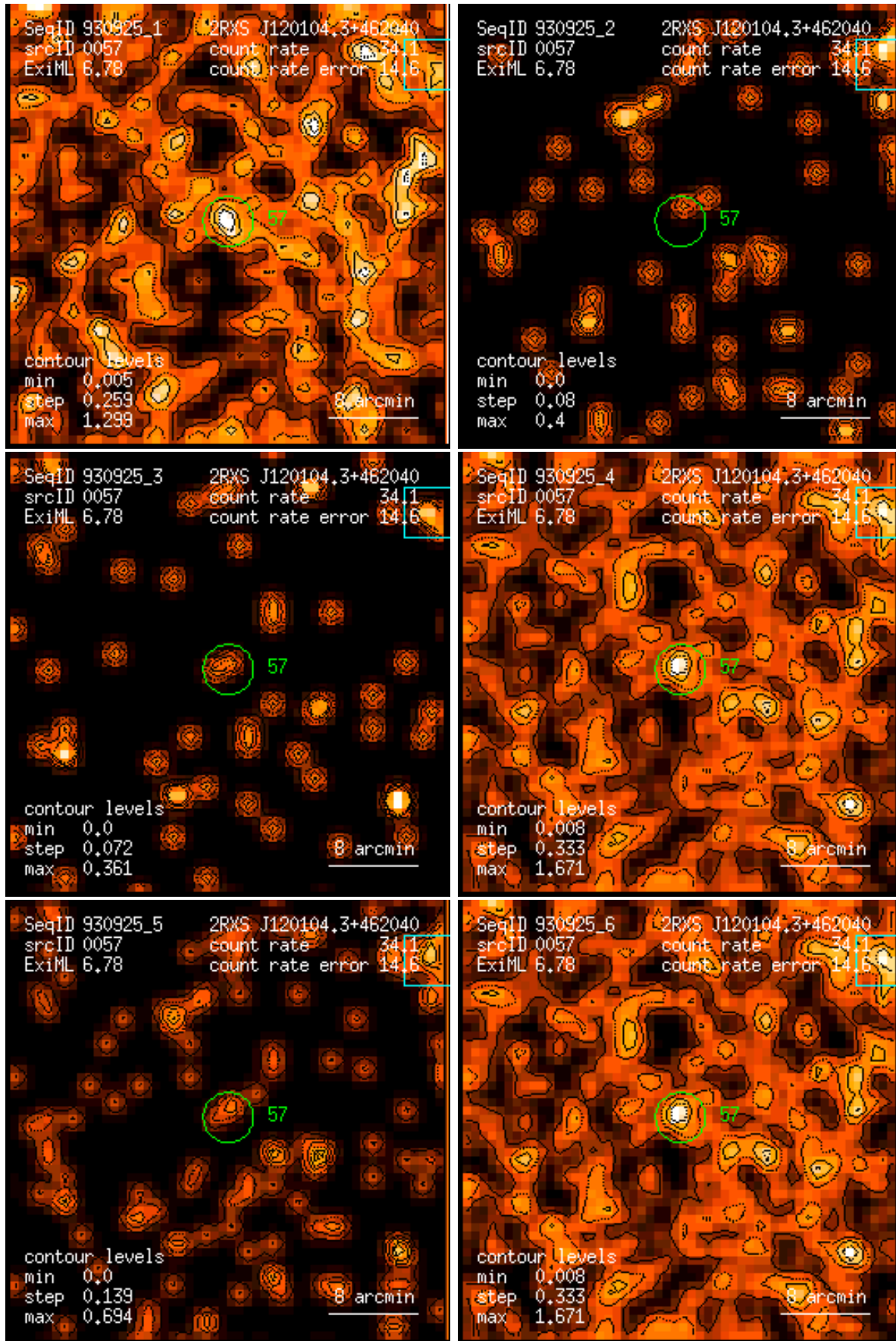
Figure 57: RASS 930925: detection 0057: band rate images, Gaussian filter: (1) PSPC channels 11 – 41, (2) 52 – 90, (3) 91 – 201, (4) 11 – 235, (5) 52 – 201, (6) 11 – 201. Broad band rates in counts/ks. Band rate contour levels in counts/ks/arcmin 2 .
