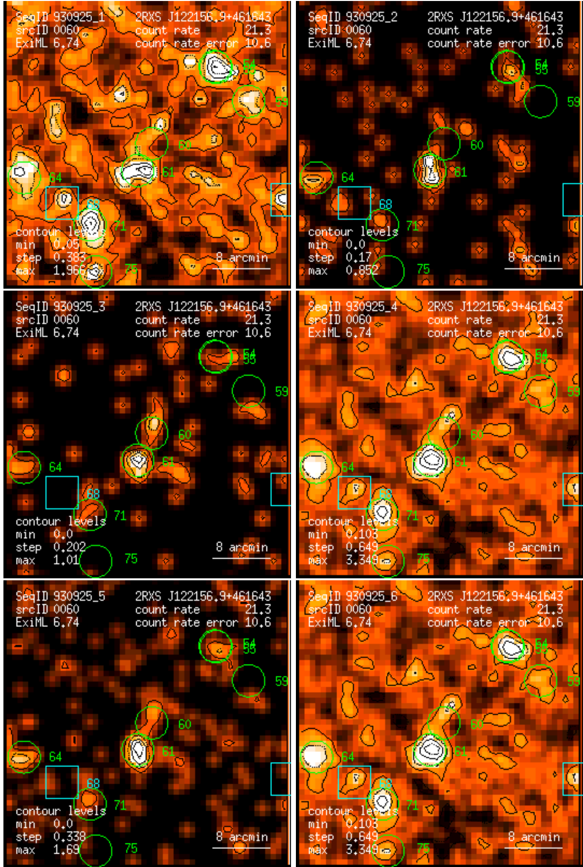
Figure 60: RASS 930925: detection 0060: band rate images, Gaussian filter: (1) PSPC channels 11 – 41, (2) 52 – 90, (3) 91 – 201, (4) 11 – 235, (5) 52 – 201, (6) 11 – 201. Broad band rates in counts/ks. Band rate contour levels in counts/ks/arcmin 2 .
