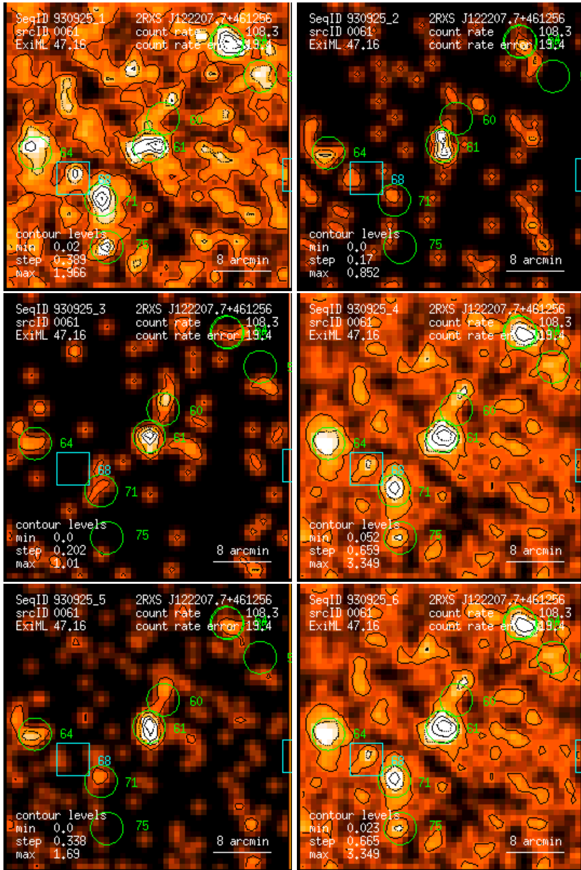
Figure 61: RASS 930925: detection 0061: band rate images, Gaussian filter: (1) PSPC channels 11 – 41, (2) 52 – 90, (3) 91 – 201, (4) 11 – 235, (5) 52 – 201, (6) 11 – 201. Broad band rates in counts/ks. Band rate contour levels in counts/ks/arcmin 2 .
