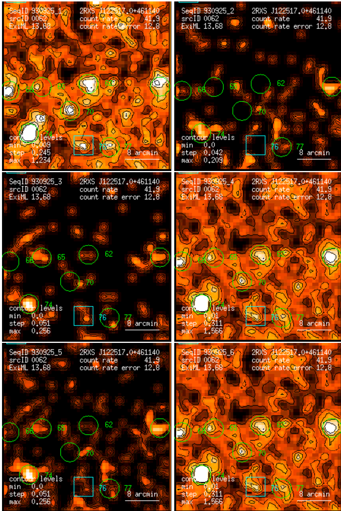
Figure 62: RASS 930925: detection 0062: band rate images, Gaussian filter: (1) PSPC channels 11 – 41, (2) 52 – 90, (3) 91 – 201, (4) 11 – 235, (5) 52 – 201, (6) 11 – 201. Broad band rates in counts/ks. Band rate contour levels in counts/ks/arcmin 2 .
