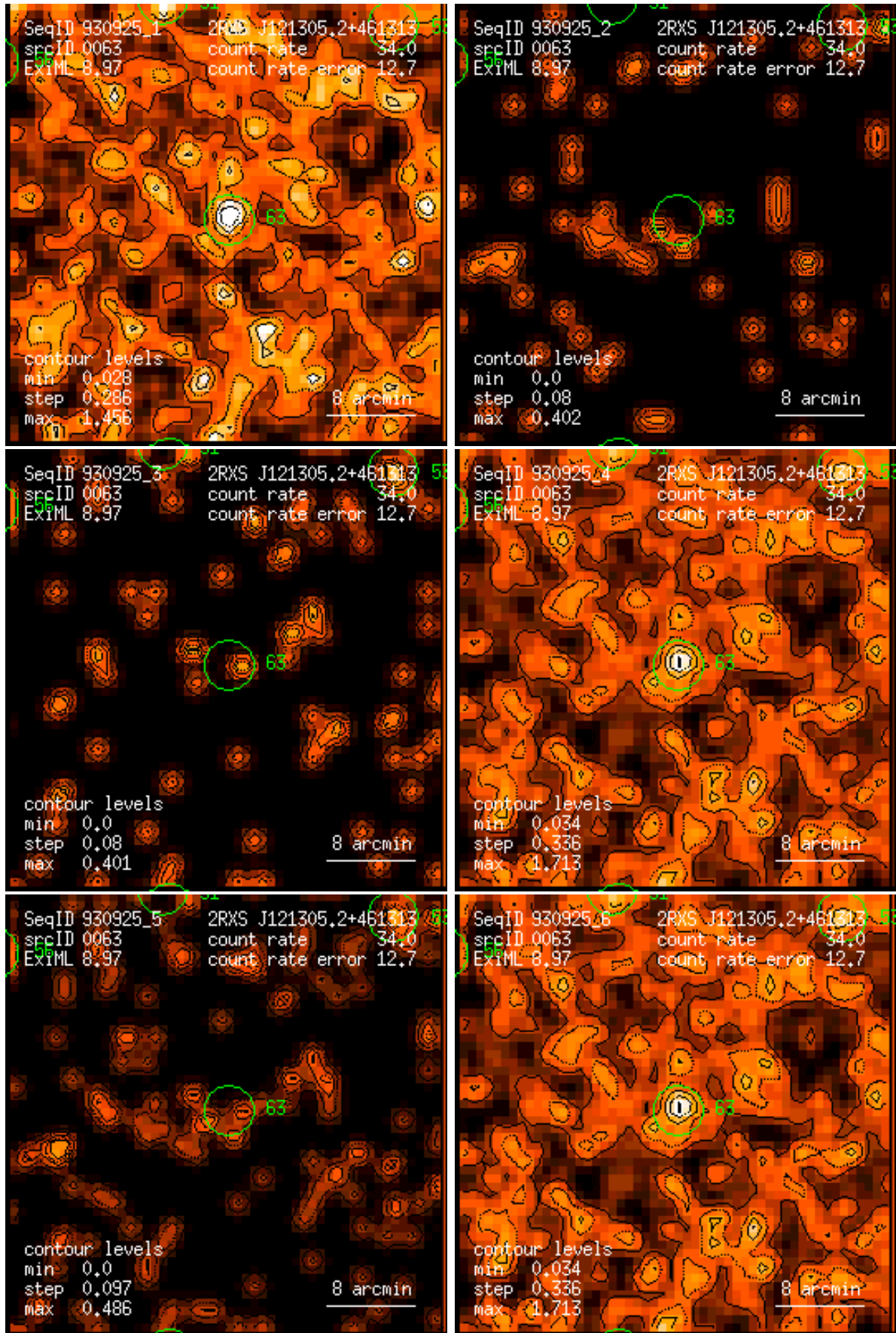
Figure 63: RASS 930925: detection 0063: band rate images, Gaussian filter: (1) PSPC channels 11 – 41, (2) 52 – 90, (3) 91 – 201, (4) 11 – 235, (5) 52 – 201, (6) 11 – 201. Broad band rates in counts/ks. Band rate contour levels in counts/ks/arcmin 2 .
