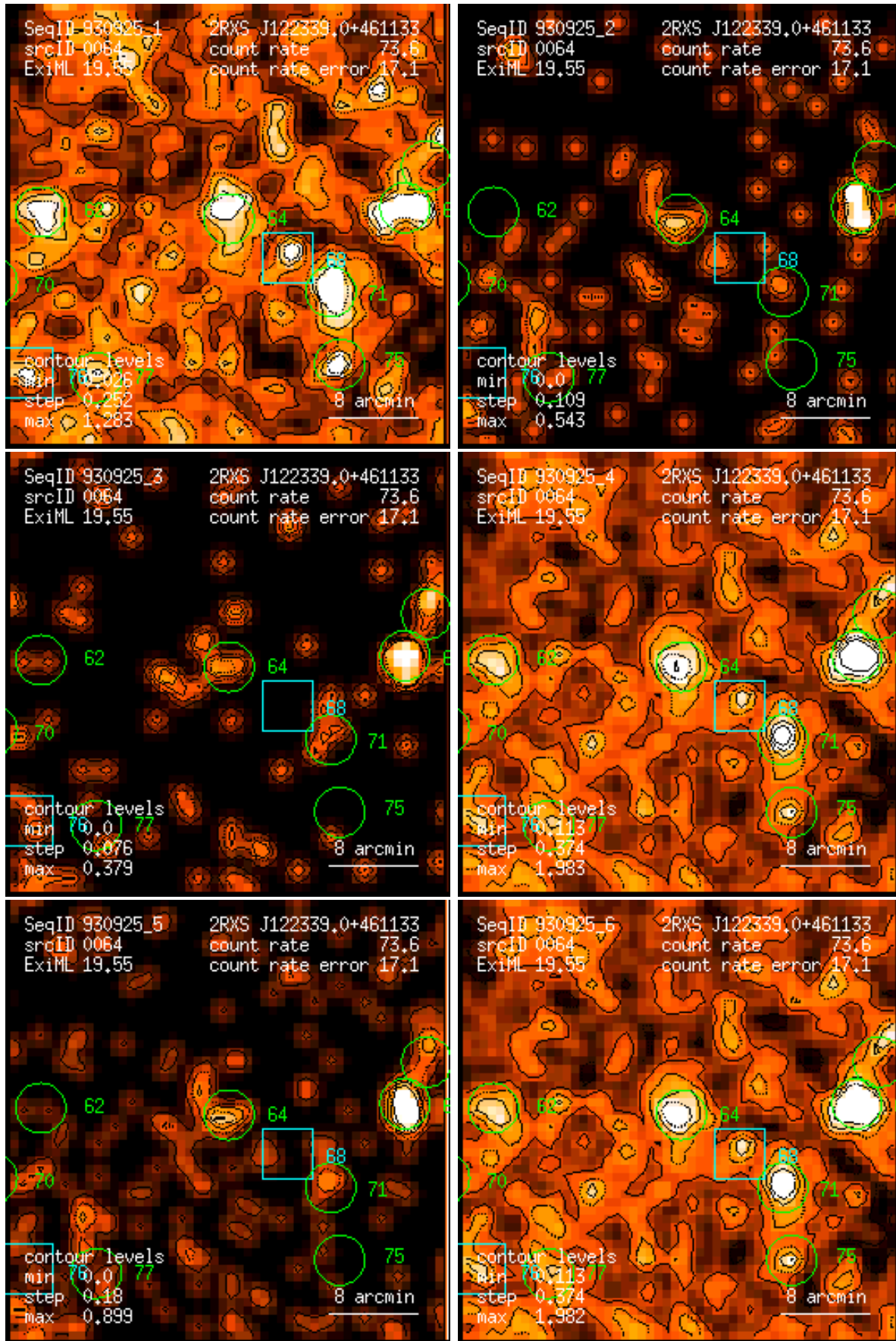
Figure 64: RASS 930925: detection 0064: band rate images, Gaussian filter: (1) PSPC channels 11 – 41, (2) 52 – 90, (3) 91 – 201, (4) 11 – 235, (5) 52 – 201, (6) 11 – 201. Broad band rates in counts/ks. Band rate contour levels in counts/ks/arcmin 2 .
