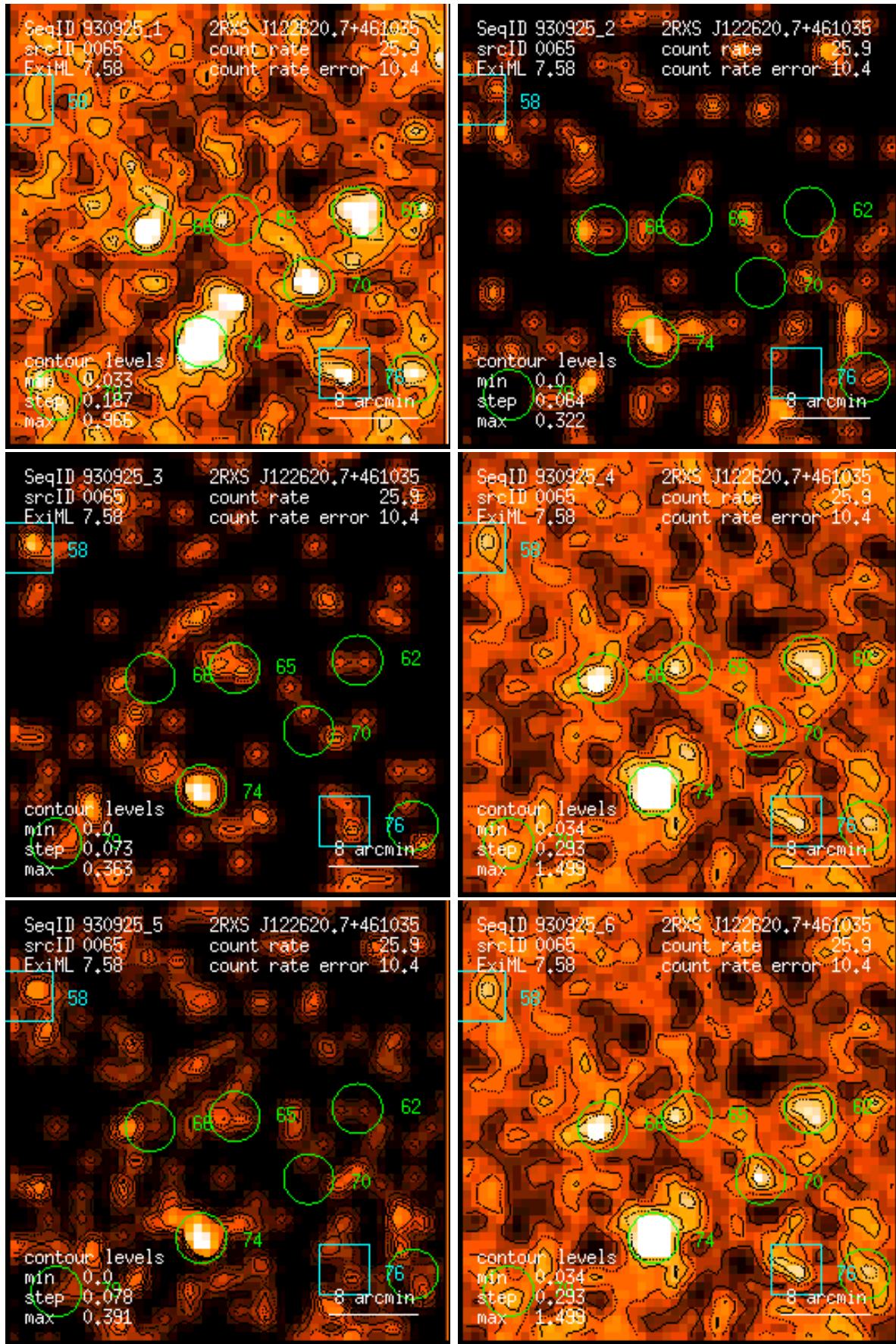
Figure 65: RASS 930925: detection 0065: band rate images, Gaussian filter: (1) PSPC channels 11 – 41, (2) 52 – 90, (3) 91 – 201, (4) 11 – 235, (5) 52 – 201, (6) 11 – 201. Broad band rates in counts/ks. Band rate contour levels in counts/ks/arcmin 2 .
