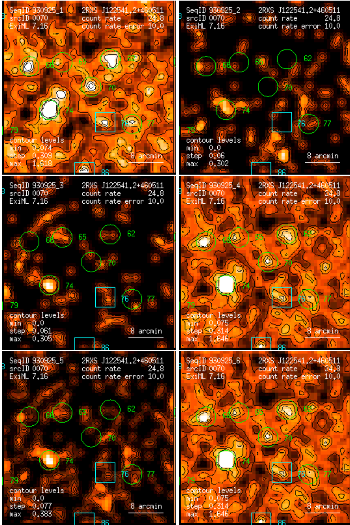
Figure 70: RASS 930925: detection 0070: band rate images, Gaussian filter: (1) PSPC channels 11 – 41, (2) 52 – 90, (3) 91 – 201, (4) 11 – 235, (5) 52 – 201, (6) 11 – 201. Broad band rates in counts/ks. Band rate contour levels in counts/ks/arcmin 2 .
