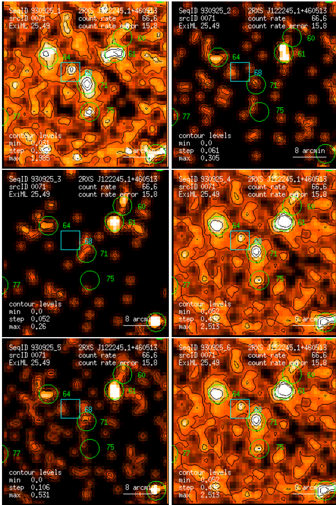
Figure 71: RASS 930925: detection 0071: band rate images, Gaussian filter: (1) PSPC channels 11 – 41, (2) 52 – 90, (3) 91 – 201, (4) 11 – 235, (5) 52 – 201, (6) 11 – 201. Broad band rates in counts/ks. Band rate contour levels in counts/ks/arcmin 2 .
