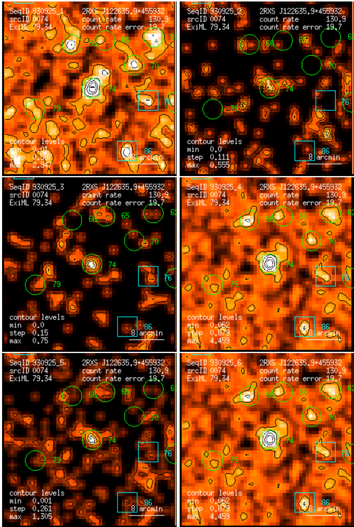
Figure 74: RASS 930925: detection 0074: band rate images, Gaussian filter: (1) PSPC channels 11 – 41, (2) 52 – 90, (3) 91 – 201, (4) 11 – 235, (5) 52 – 201, (6) 11 – 201. Broad band rates in counts/ks. Band rate contour levels in counts/ks/arcmin 2 .
