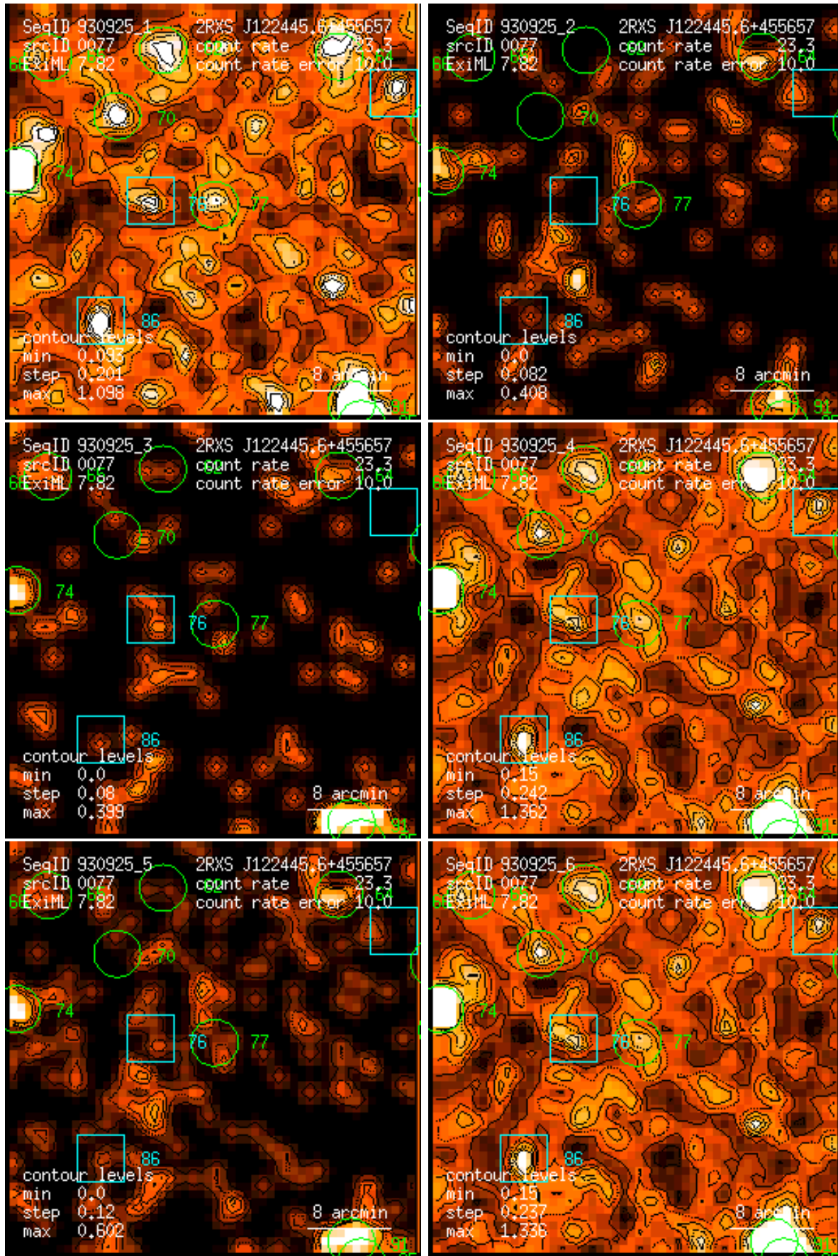
Figure 77: RASS 930925: detection 0077: band rate images, Gaussian filter: (1) PSPC channels 11 – 41, (2) 52 – 90, (3) 91 – 201, (4) 11 – 235, (5) 52 – 201, (6) 11 – 201. Broad band rates in counts/ks. Band rate contour levels in counts/ks/arcmin 2 .
