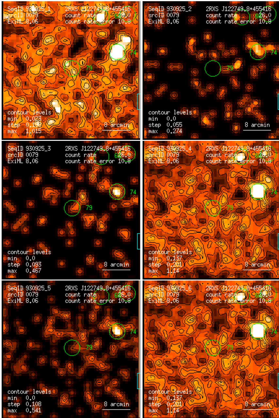
Figure 79: RASS 930925: detection 0079: band rate images, Gaussian filter: (1) PSPC channels 11 – 41, (2) 52 – 90, (3) 91 – 201, (4) 11 – 235, (5) 52 – 201, (6) 11 – 201. Broad band rates in counts/ks. Band rate contour levels in counts/ks/arcmin 2 .
