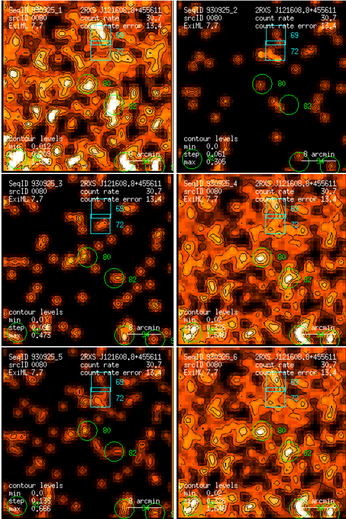
Figure 80: RASS 930925: detection 0080: band rate images, Gaussian filter: (1) PSPC channels 11 – 41, (2) 52 – 90, (3) 91 – 201, (4) 11 – 235, (5) 52 – 201, (6) 11 – 201. Broad band rates in counts/ks. Band rate contour levels in counts/ks/arcmin 2 .
