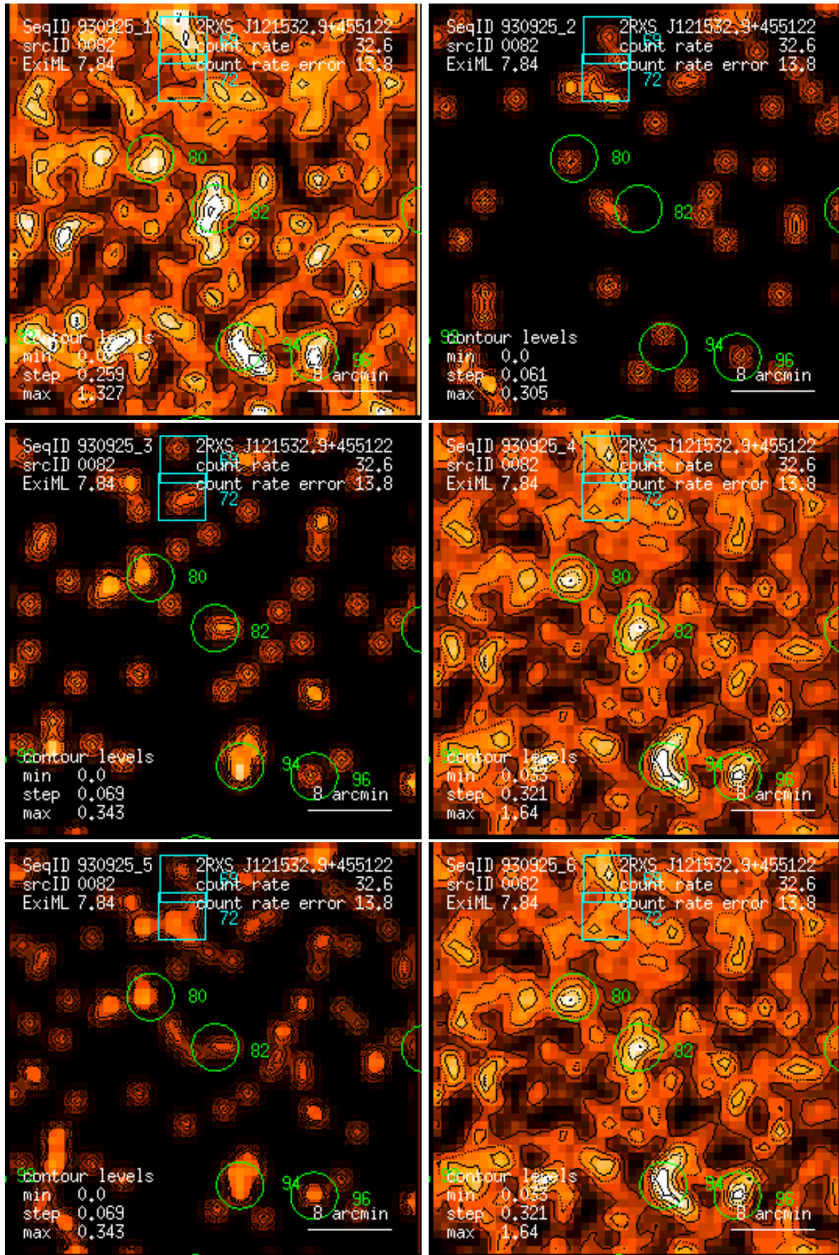
Figure 82: RASS 930925: detection 0082: band rate images, Gaussian filter: (1) PSPC channels 11 – 41, (2) 52 – 90, (3) 91 – 201, (4) 11 – 235, (5) 52 – 201, (6) 11 – 201. Broad band rates in counts/ks. Band rate contour levels in counts/ks/arcmin 2 .
