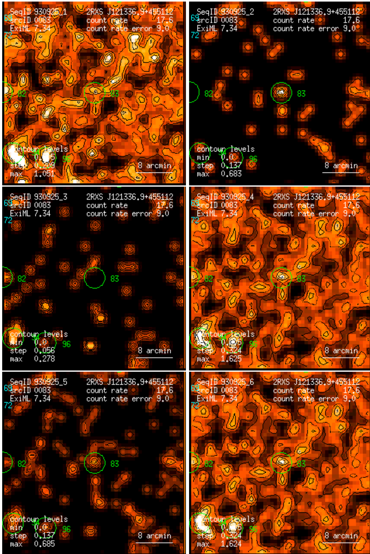
Figure 83: RASS 930925: detection 0083: band rate images, Gaussian filter: (1) PSPC channels 11 – 41, (2) 52 – 90, (3) 91 – 201, (4) 11 – 235, (5) 52 – 201, (6) 11 – 201. Broad band rates in counts/ks. Band rate contour levels in counts/ks/arcmin 2 .
