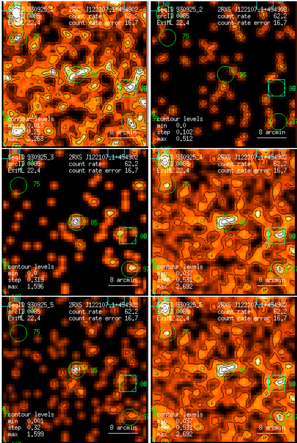
Figure 85: RASS 930925: detection 0085: band rate images, Gaussian filter: (1) PSPC channels 11 – 41, (2) 52 – 90, (3) 91 – 201, (4) 11 – 235, (5) 52 – 201, (6) 11 – 201. Broad band rates in counts/ks. Band rate contour levels in counts/ks/arcmin 2 .
