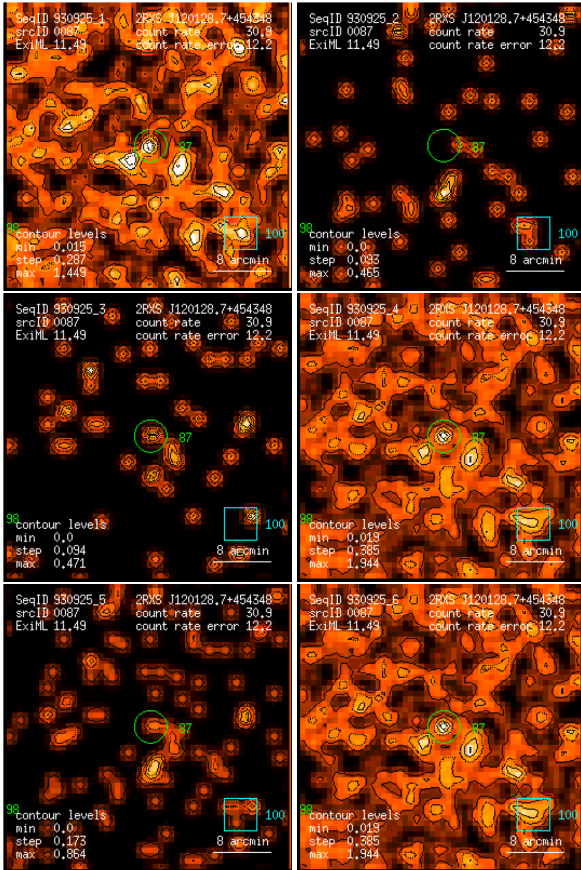
Figure 87: RASS 930925: detection 0087: band rate images, Gaussian filter: (1) PSPC channels 11 – 41, (2) 52 – 90, (3) 91 – 201, (4) 11 – 235, (5) 52 – 201, (6) 11 – 201. Broad band rates in counts/ks. Band rate contour levels in counts/ks/arcmin 2 .
