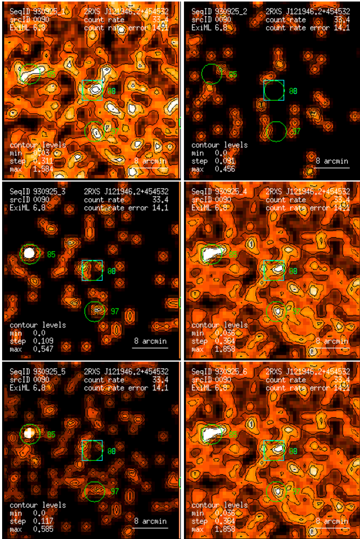
Figure 90: RASS 930925: detection 0090: band rate images, Gaussian filter: (1) PSPC channels 11 – 41, (2) 52 – 90, (3) 91 – 201, (4) 11 – 235, (5) 52 – 201, (6) 11 – 201. Broad band rates in counts/ks. Band rate contour levels in counts/ks/arcmin 2 .
