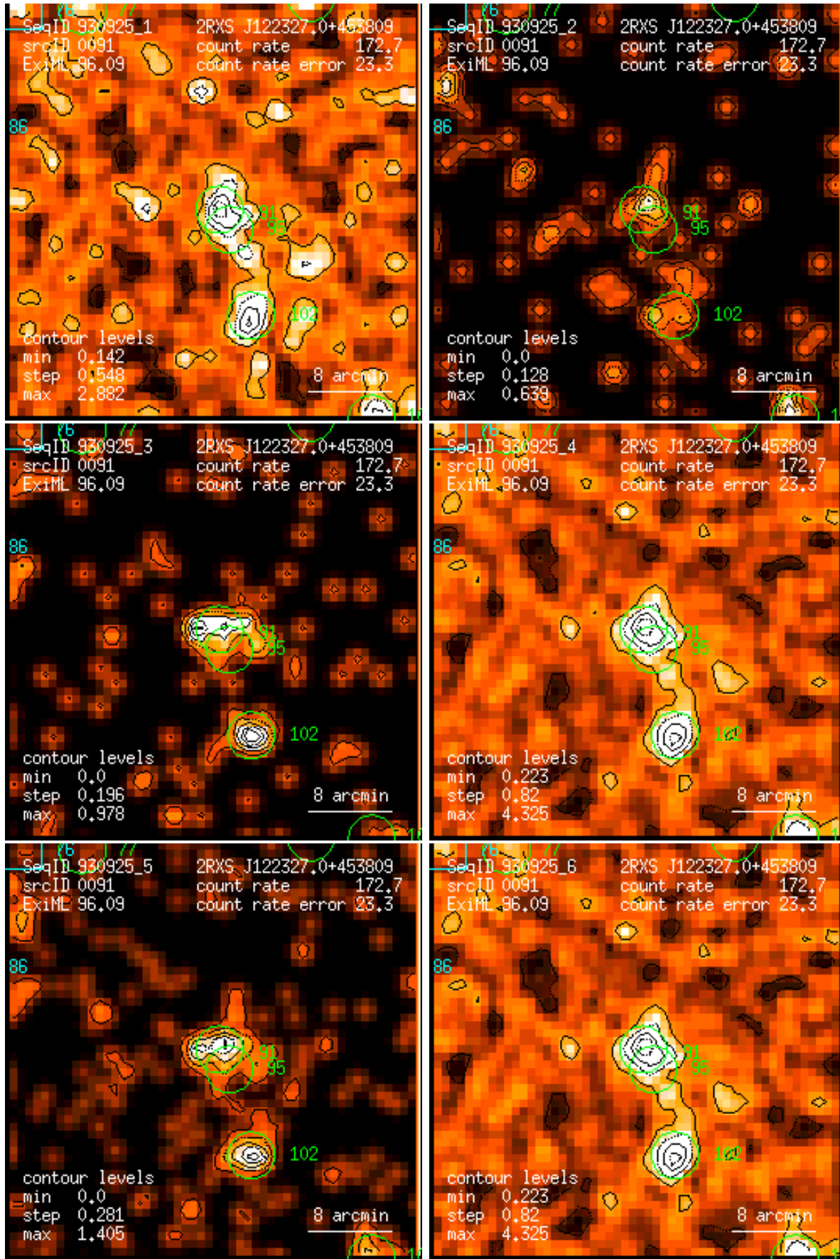
Figure 91: RASS 930925: detection 0091: band rate images, Gaussian filter: (1) PSPC channels 11 – 41, (2) 52 – 90, (3) 91 – 201, (4) 11 – 235, (5) 52 – 201, (6) 11 – 201. Broad band rates in counts/ks. Band rate contour levels in counts/ks/arcmin 2 .
