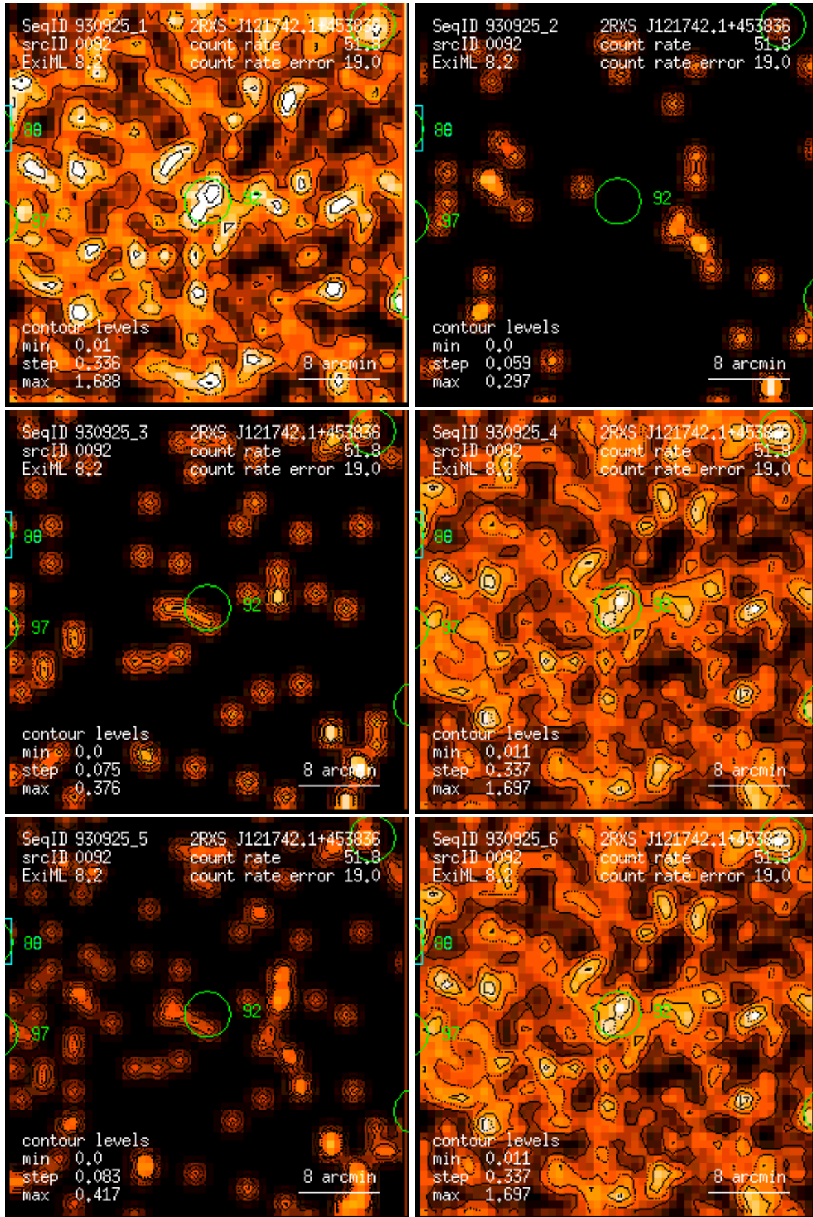
Figure 92: RASS 930925: detection 0092: band rate images, Gaussian filter: (1) PSPC channels 11 – 41, (2) 52 – 90, (3) 91 – 201, (4) 11 – 235, (5) 52 – 201, (6) 11 – 201. Broad band rates in counts/ks. Band rate contour levels in counts/ks/arcmin 2 .
