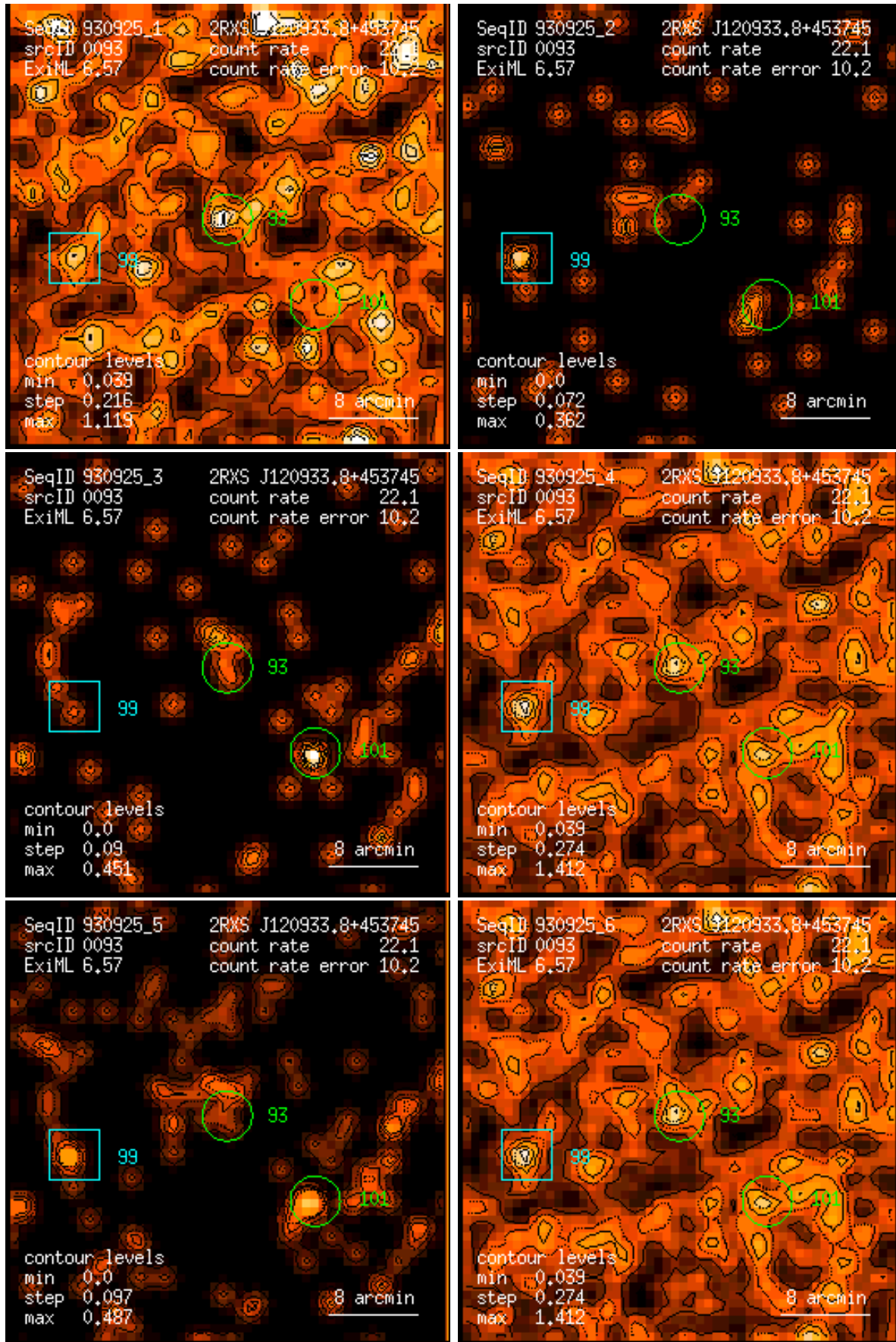
Figure 93: RASS 930925: detection 0093: band rate images, Gaussian filter: (1) PSPC channels 11 – 41, (2) 52 – 90, (3) 91 – 201, (4) 11 – 235, (5) 52 – 201, (6) 11 – 201. Broad band rates in counts/ks. Band rate contour levels in counts/ks/arcmin 2 .
