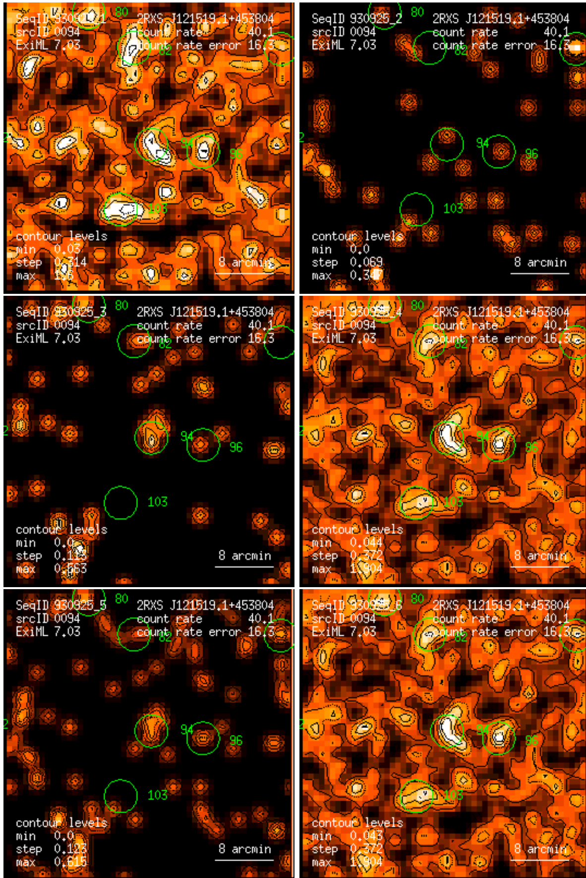
Figure 94: RASS 930925: detection 0094: band rate images, Gaussian filter: (1) PSPC channels 11 – 41, (2) 52 – 90, (3) 91 – 201, (4) 11 – 235, (5) 52 – 201, (6) 11 – 201. Broad band rates in counts/ks. Band rate contour levels in counts/ks/arcmin 2 .
