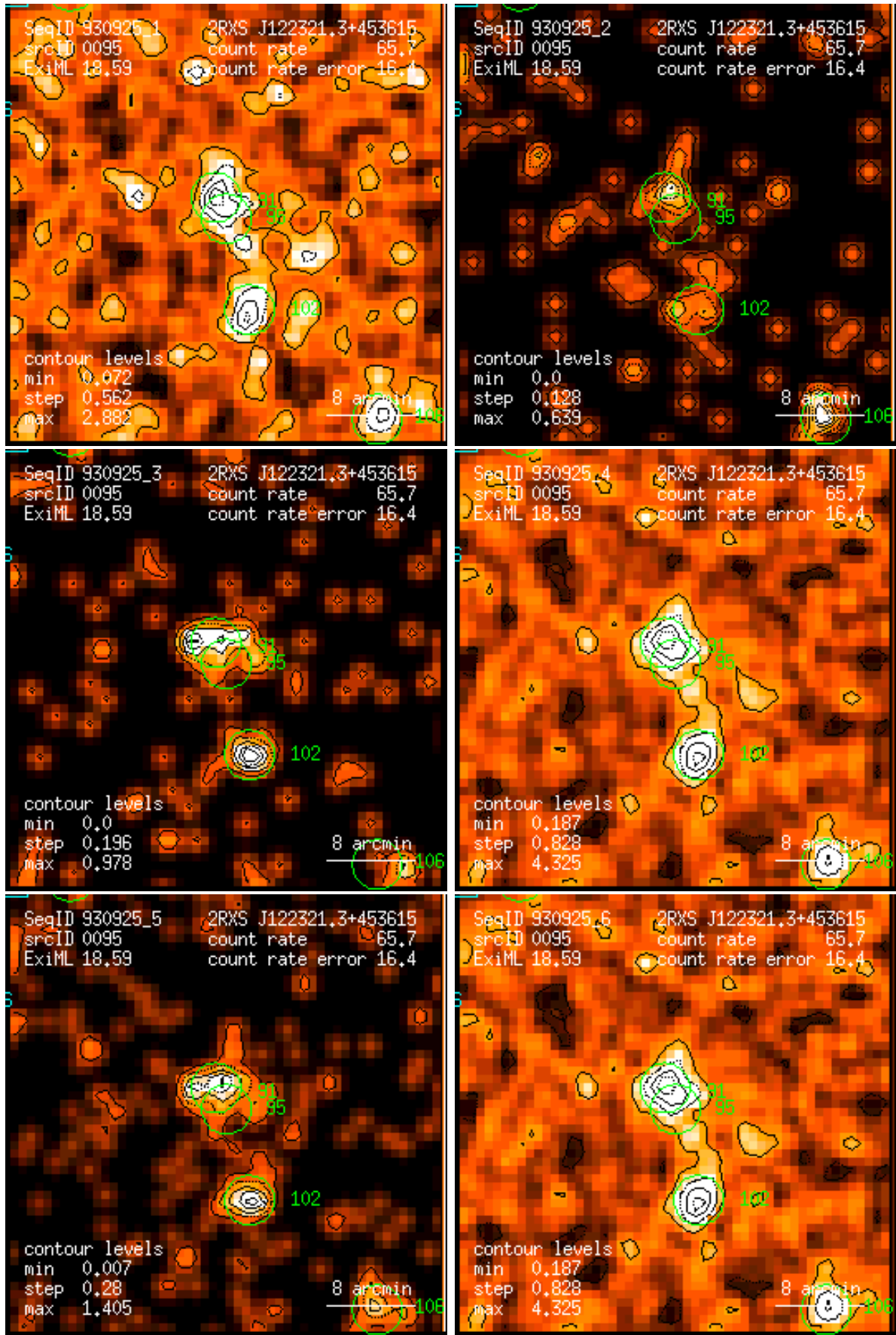
Figure 95: RASS 930925: detection 0095: band rate images, Gaussian filter: (1) PSPC channels 11 – 41, (2) 52 – 90, (3) 91 – 201, (4) 11 – 235, (5) 52 – 201, (6) 11 – 201. Broad band rates in counts/ks. Band rate contour levels in counts/ks/arcmin 2 .
