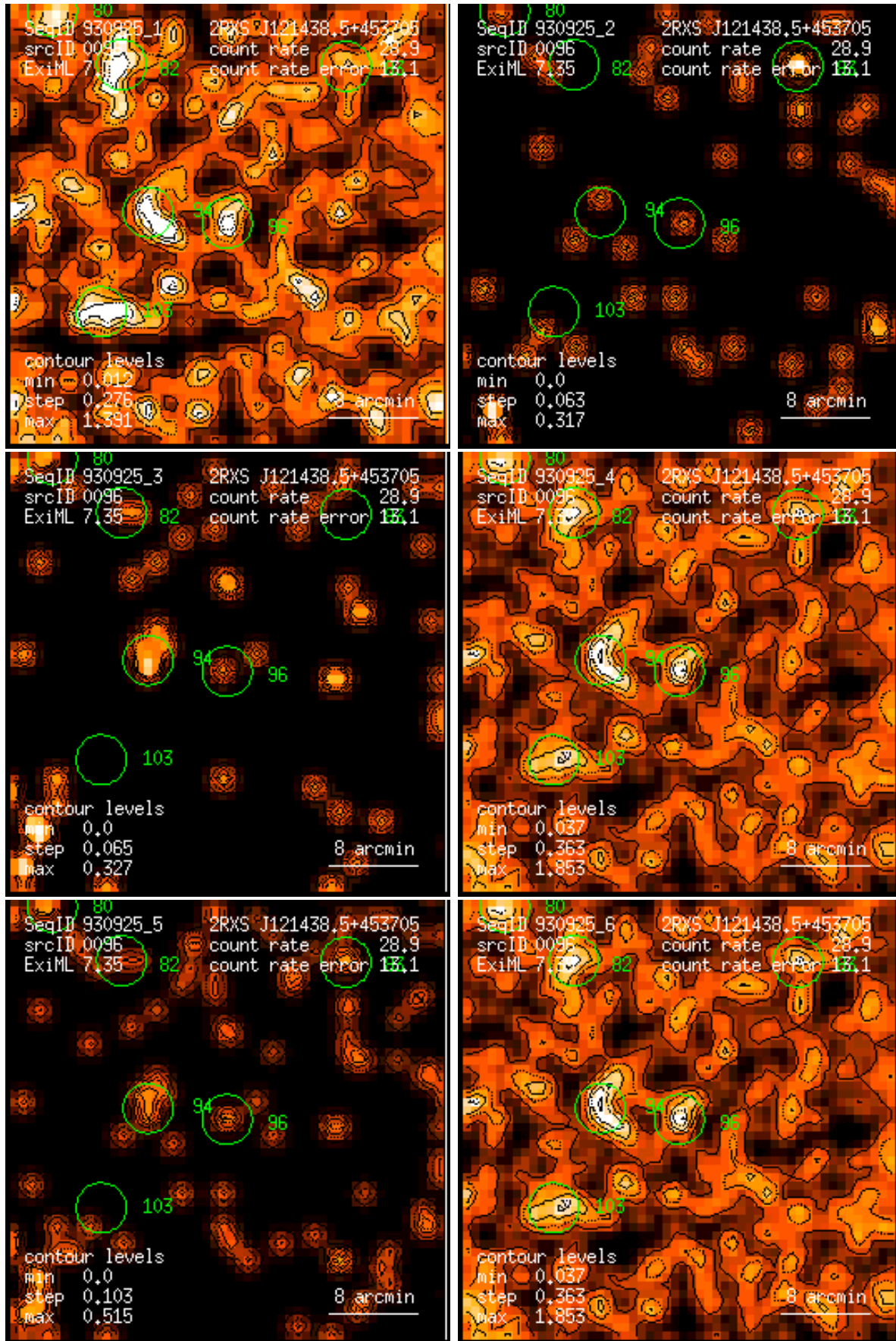
Figure 96: RASS 930925: detection 0096: band rate images, Gaussian filter: (1) PSPC channels 11 – 41, (2) 52 – 90, (3) 91 – 201, (4) 11 – 235, (5) 52 – 201, (6) 11 – 201. Broad band rates in counts/ks. Band rate contour levels in counts/ks/arcmin 2 .
