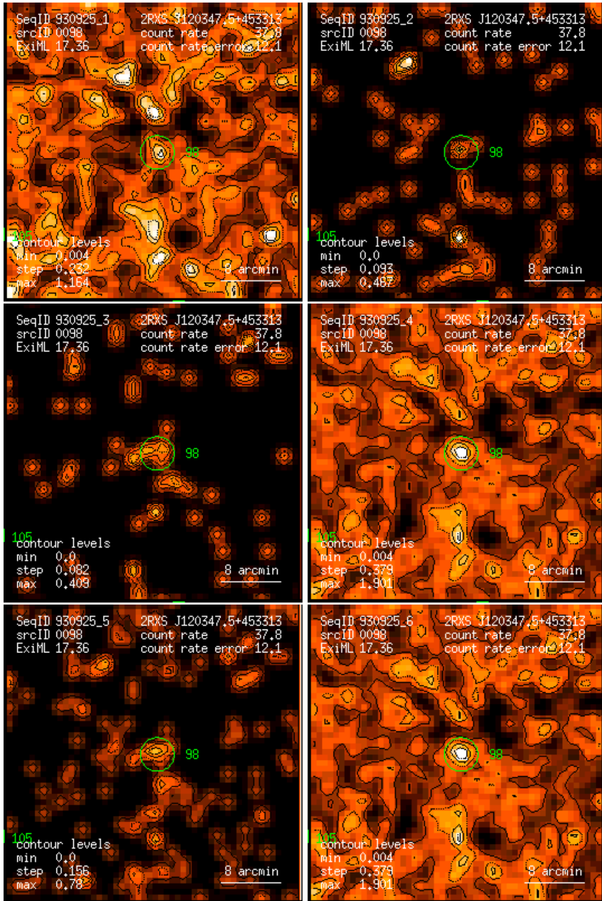
Figure 98: RASS 930925: detection 0098: band rate images, Gaussian filter: (1) PSPC channels 11 – 41, (2) 52 – 90, (3) 91 – 201, (4) 11 – 235, (5) 52 – 201, (6) 11 – 201. Broad band rates in counts/ks. Band rate contour levels in counts/ks/arcmin 2 .
