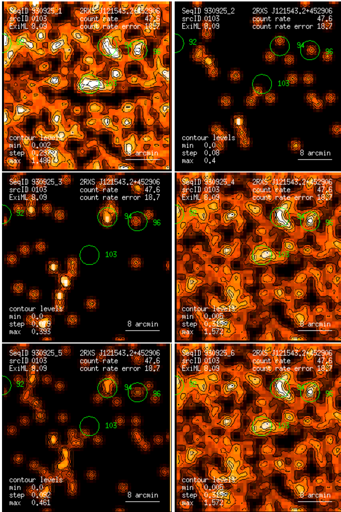
Figure 103: RASS 930925: detection 0103: band rate images, Gaussian filter: (1) PSPC channels 11 – 41, (2) 52 – 90, (3) 91 – 201, (4) 11 – 235, (5) 52 – 201, (6) 11 – 201. Broad band rates in counts/ks. Band rate contour levels in counts/ks/arcmin 2 .
