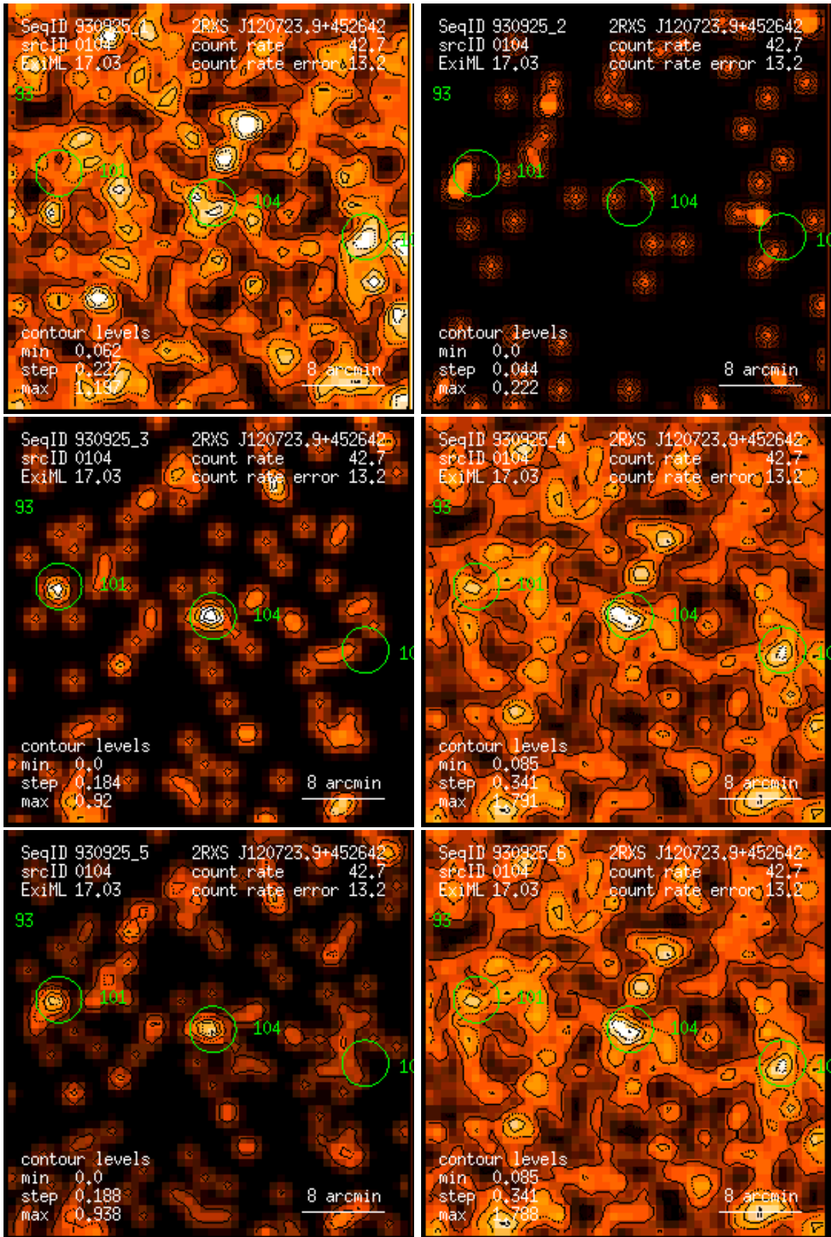
Figure 104: RASS 930925: detection 0104: band rate images, Gaussian filter: (1) PSPC channels 11 – 41, (2) 52 – 90, (3) 91 – 201, (4) 11 – 235, (5) 52 – 201, (6) 11 – 201. Broad band rates in counts/ks. Band rate contour levels in counts/ks/arcmin 2 .
