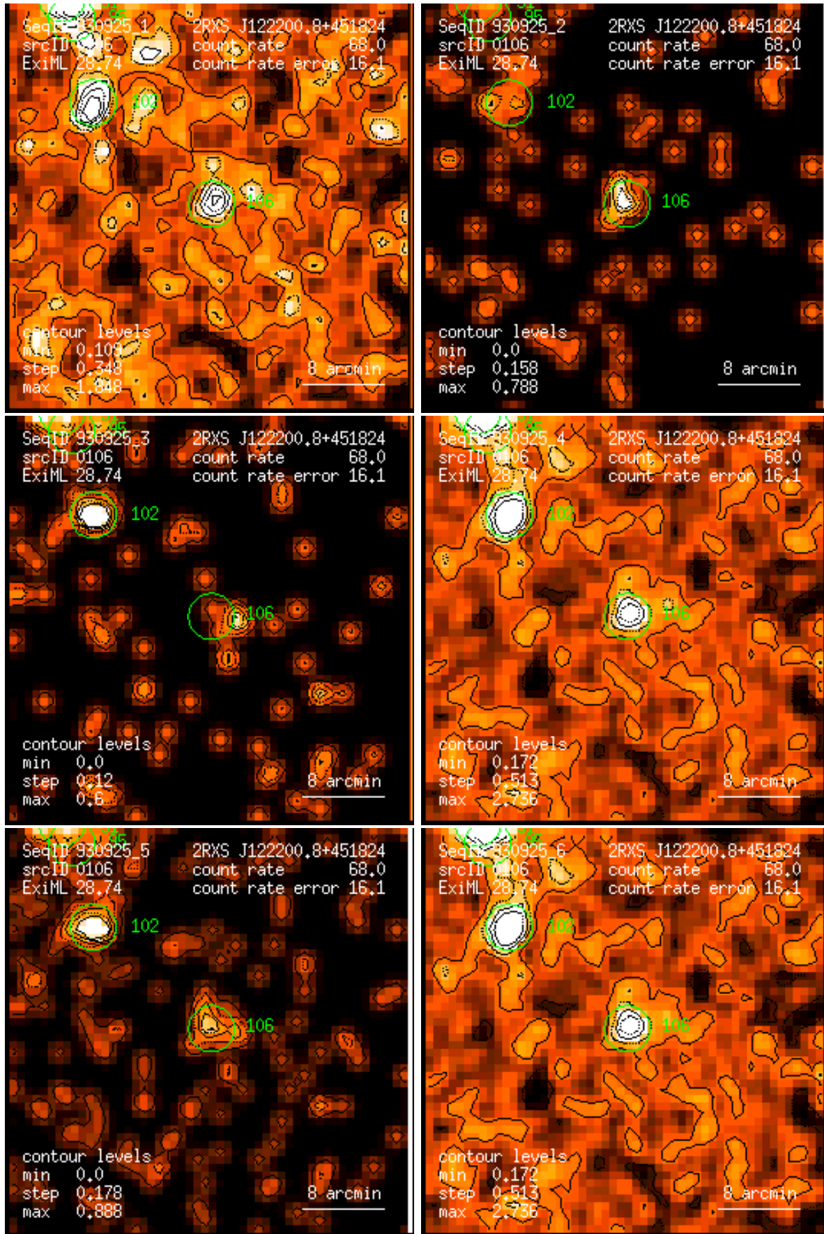
Figure 106: RASS 930925: detection 0106: band rate images, Gaussian filter: (1) PSPC channels 11 – 41, (2) 52 – 90, (3) 91 – 201, (4) 11 – 235, (5) 52 – 201, (6) 11 – 201. Broad band rates in counts/ks. Band rate contour levels in counts/ks/arcmin 2 .
