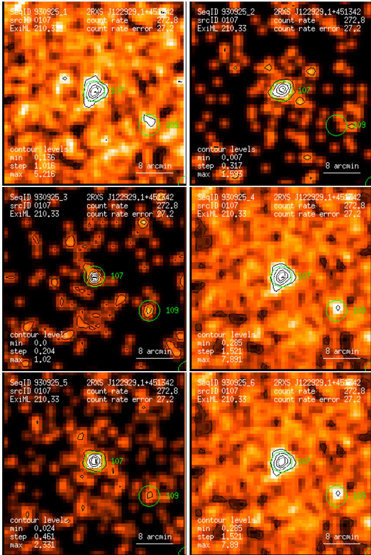
Figure 107: RASS 930925: detection 0107: band rate images, Gaussian filter: (1) PSPC channels 11 – 41, (2) 52 – 90, (3) 91 – 201, (4) 11 – 235, (5) 52 – 201, (6) 11 – 201. Broad band rates in counts/ks. Band rate contour levels in counts/ks/arcmin 2 .
