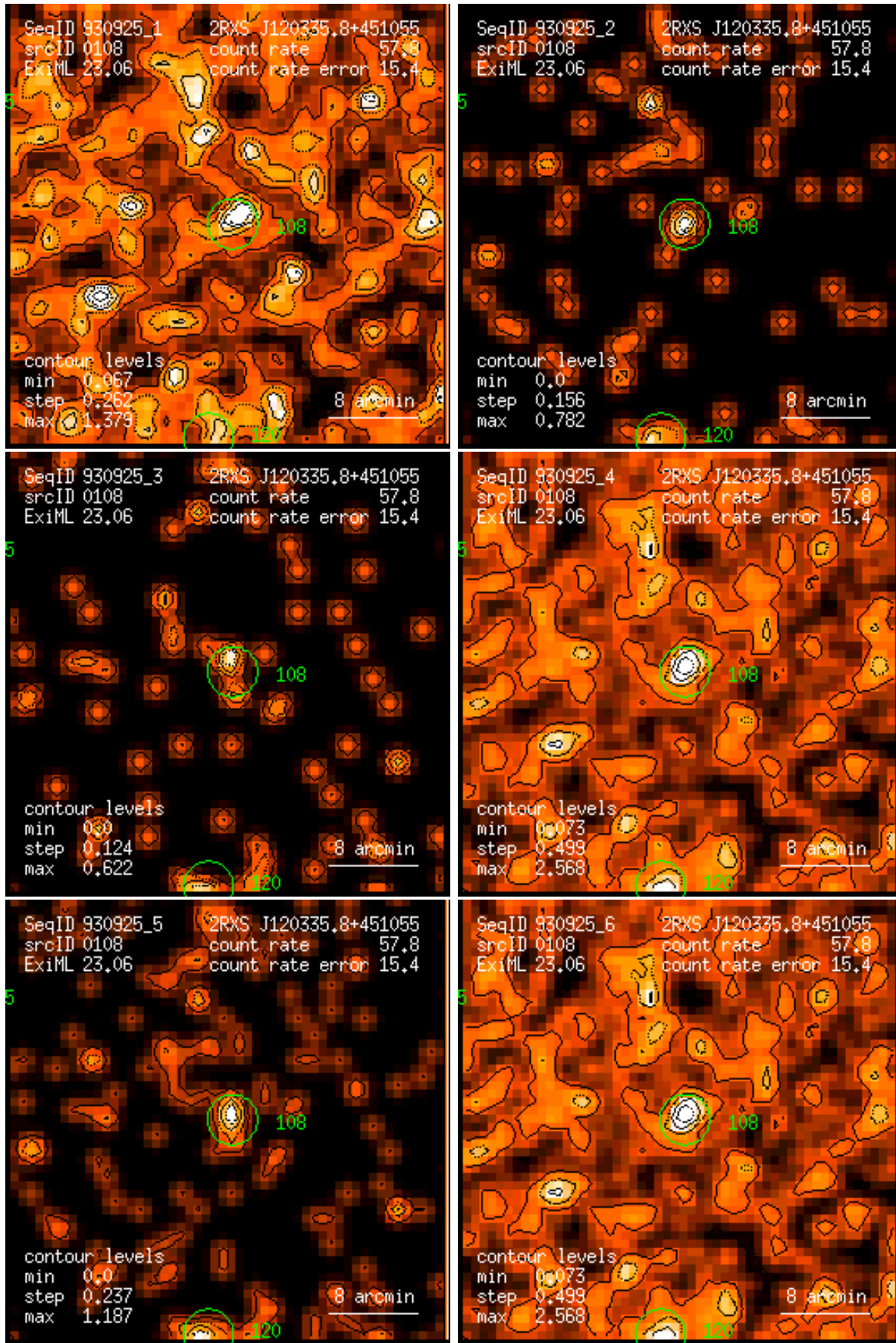
Figure 108: RASS 930925: detection 0108: band rate images, Gaussian filter: (1) PSPC channels 11 – 41, (2) 52 – 90, (3) 91 – 201, (4) 11 – 235, (5) 52 – 201, (6) 11 – 201. Broad band rates in counts/ks. Band rate contour levels in counts/ks/arcmin 2 .
