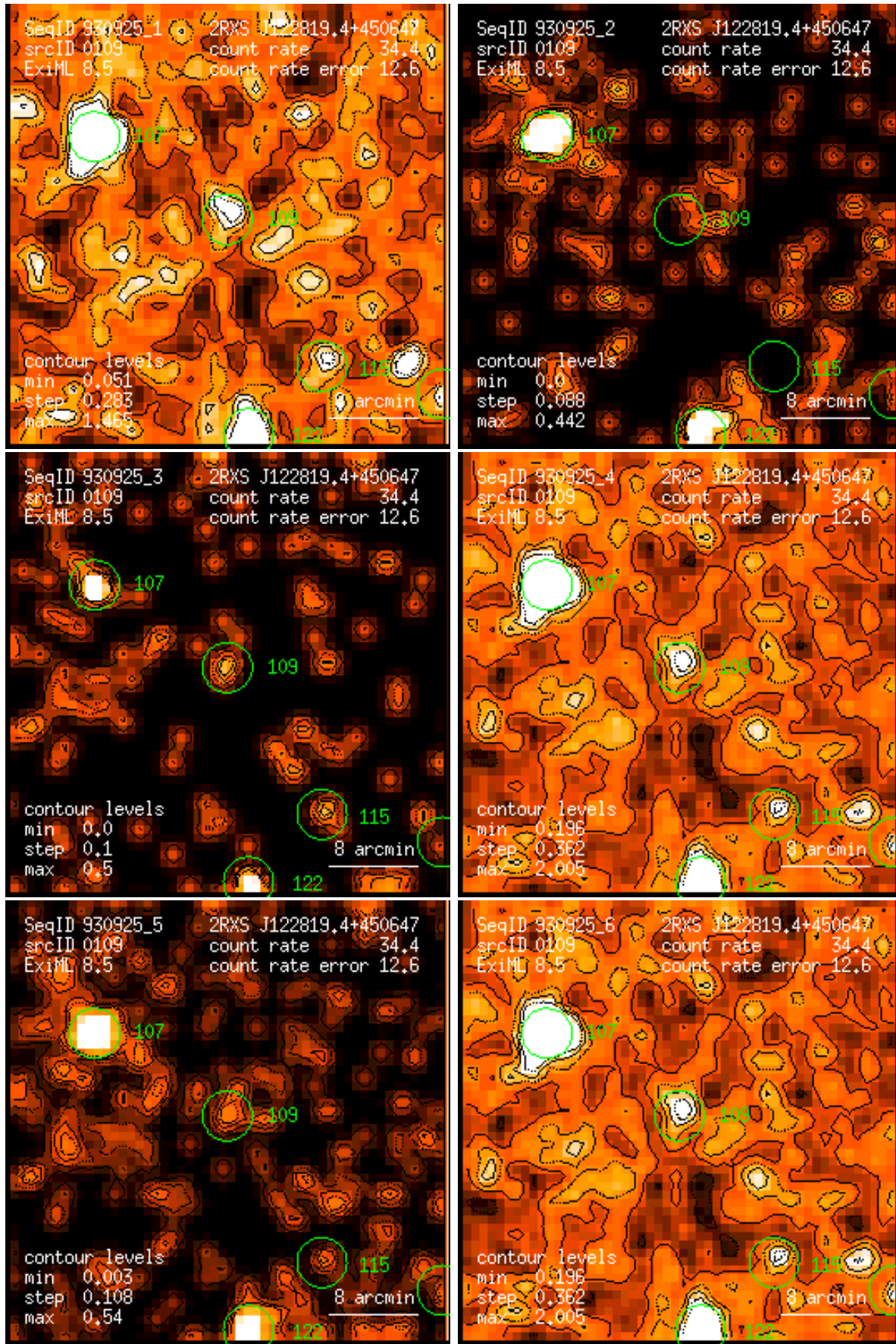
Figure 109: RASS 930925: detection 0109: band rate images, Gaussian filter: (1) PSPC channels 11 – 41, (2) 52 – 90, (3) 91 – 201, (4) 11 – 235, (5) 52 – 201, (6) 11 – 201. Broad band rates in counts/ks. Band rate contour levels in counts/ks/arcmin 2 .
