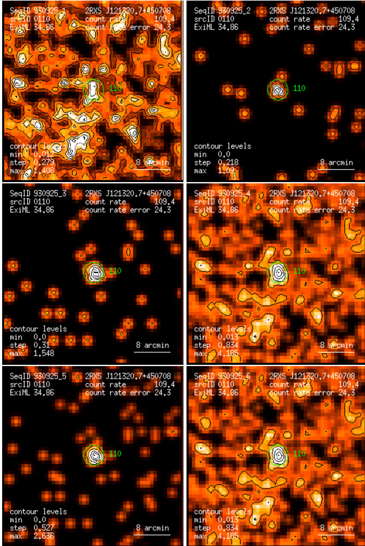
Figure 110: RASS 930925: detection 0110: band rate images, Gaussian filter: (1) PSPC channels 11 – 41, (2) 52 – 90, (3) 91 – 201, (4) 11 – 235, (5) 52 – 201, (6) 11 – 201. Broad band rates in counts/ks. Band rate contour levels in counts/ks/arcmin 2 .
