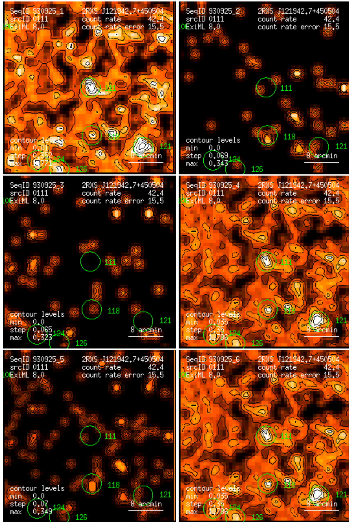
Figure 111: RASS 930925: detection 0111: band rate images, Gaussian filter: (1) PSPC channels 11 – 41, (2) 52 – 90, (3) 91 – 201, (4) 11 – 235, (5) 52 – 201, (6) 11 – 201. Broad band rates in counts/ks. Band rate contour levels in counts/ks/arcmin 2 .
