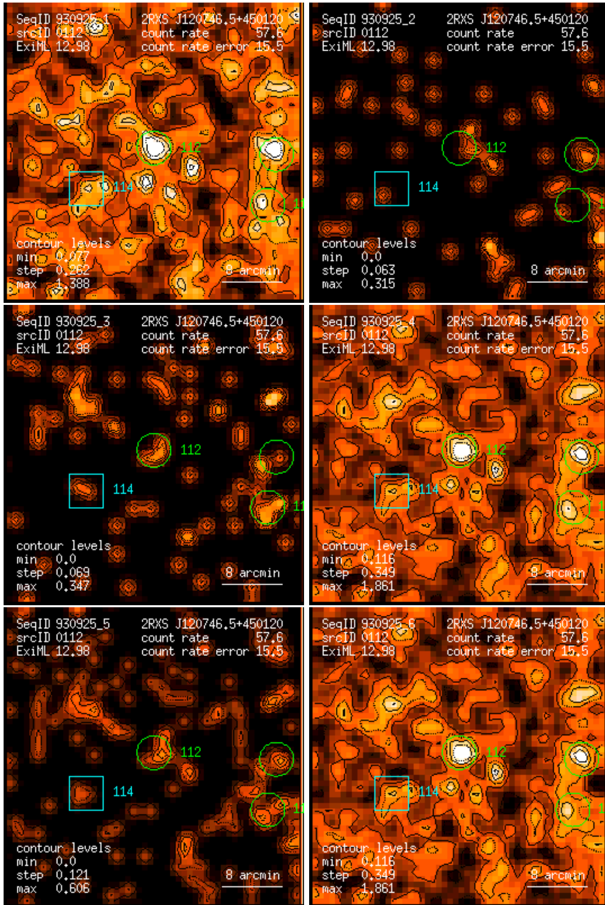
Figure 112: RASS 930925: detection 0112: band rate images, Gaussian filter: (1) PSPC channels 11 – 41, (2) 52 – 90, (3) 91 – 201, (4) 11 – 235, (5) 52 – 201, (6) 11 – 201. Broad band rates in counts/ks. Band rate contour levels in counts/ks/arcmin 2 .
