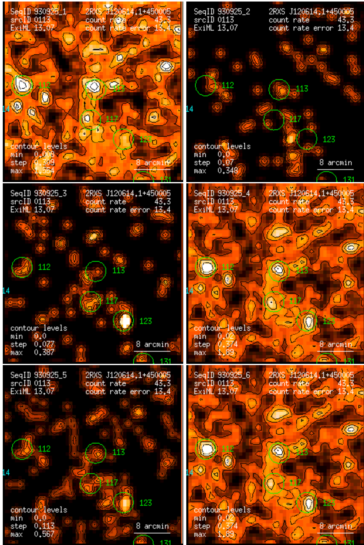
Figure 113: RASS 930925: detection 0113: band rate images, Gaussian filter: (1) PSPC channels 11 – 41, (2) 52 – 90, (3) 91 – 201, (4) 11 – 235, (5) 52 – 201, (6) 11 – 201. Broad band rates in counts/ks. Band rate contour levels in counts/ks/arcmin 2 .
