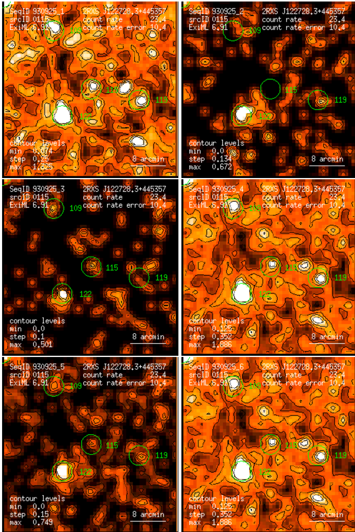
Figure 115: RASS 930925: detection 0115: band rate images, Gaussian filter: (1) PSPC channels 11 – 41, (2) 52 – 90, (3) 91 – 201, (4) 11 – 235, (5) 52 – 201, (6) 11 – 201. Broad band rates in counts/ks. Band rate contour levels in counts/ks/arcmin 2 .
