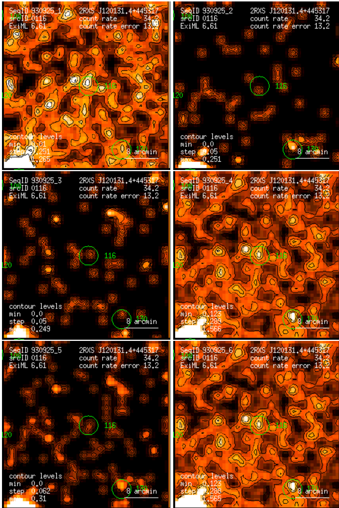
Figure 116: RASS 930925: detection 0116: band rate images, Gaussian filter: (1) PSPC channels 11 – 41, (2) 52 – 90, (3) 91 – 201, (4) 11 – 235, (5) 52 – 201, (6) 11 – 201. Broad band rates in counts/ks. Band rate contour levels in counts/ks/arcmin 2 .
