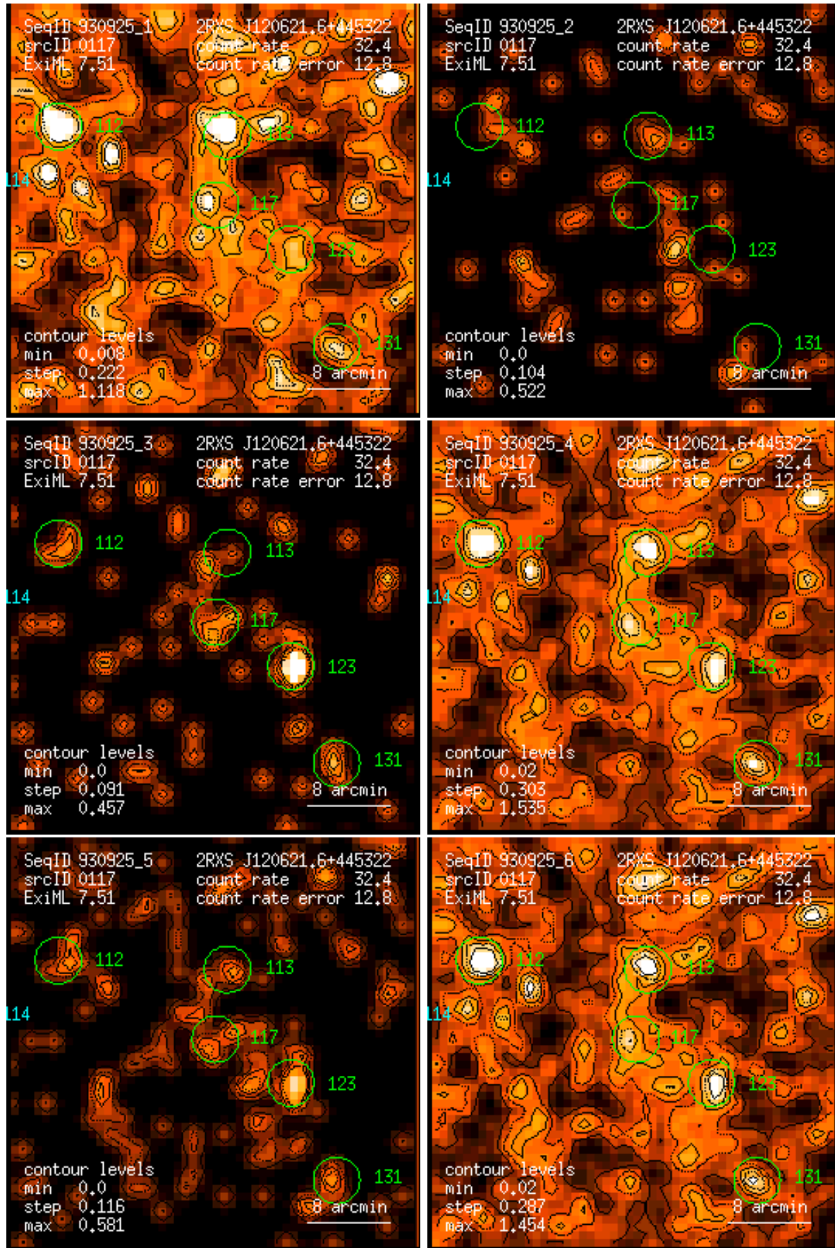
Figure 117: RASS 930925: detection 0117: band rate images, Gaussian filter: (1) PSPC channels 11 – 41, (2) 52 – 90, (3) 91 – 201, (4) 11 – 235, (5) 52 – 201, (6) 11 – 201. Broad band rates in counts/ks. Band rate contour levels in counts/ks/arcmin 2 .
