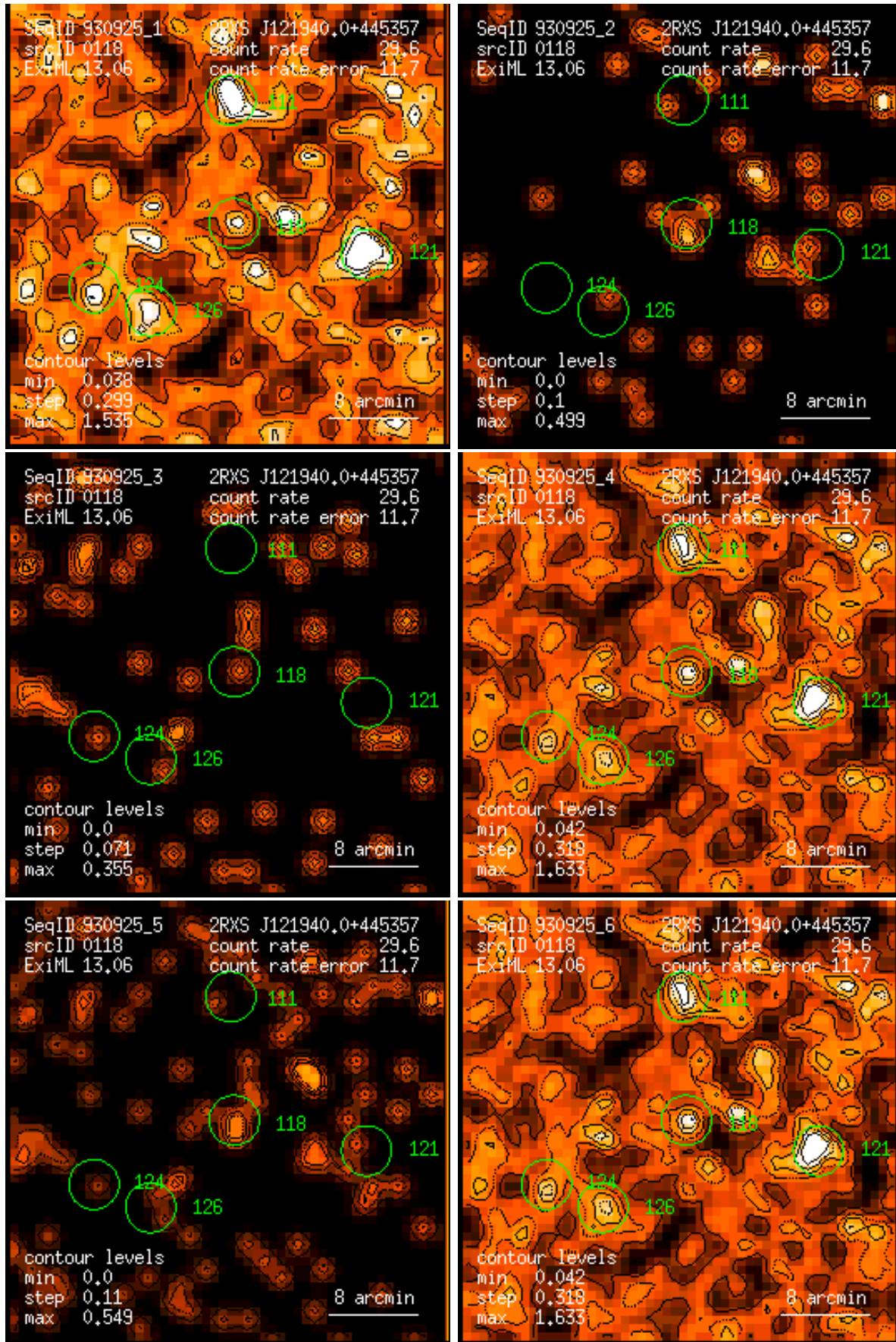
Figure 118: RASS 930925: detection 0118: band rate images, Gaussian filter: (1) PSPC channels 11 – 41, (2) 52 – 90, (3) 91 – 201, (4) 11 – 235, (5) 52 – 201, (6) 11 – 201. Broad band rates in counts/ks. Band rate contour levels in counts/ks/arcmin 2 .
