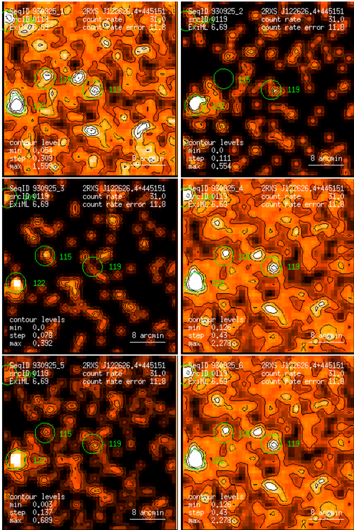
Figure 119: RASS 930925: detection 0119: band rate images, Gaussian filter: (1) PSPC channels 11 – 41, (2) 52 – 90, (3) 91 – 201, (4) 11 – 235, (5) 52 – 201, (6) 11 – 201. Broad band rates in counts/ks. Band rate contour levels in counts/ks/arcmin 2 .
