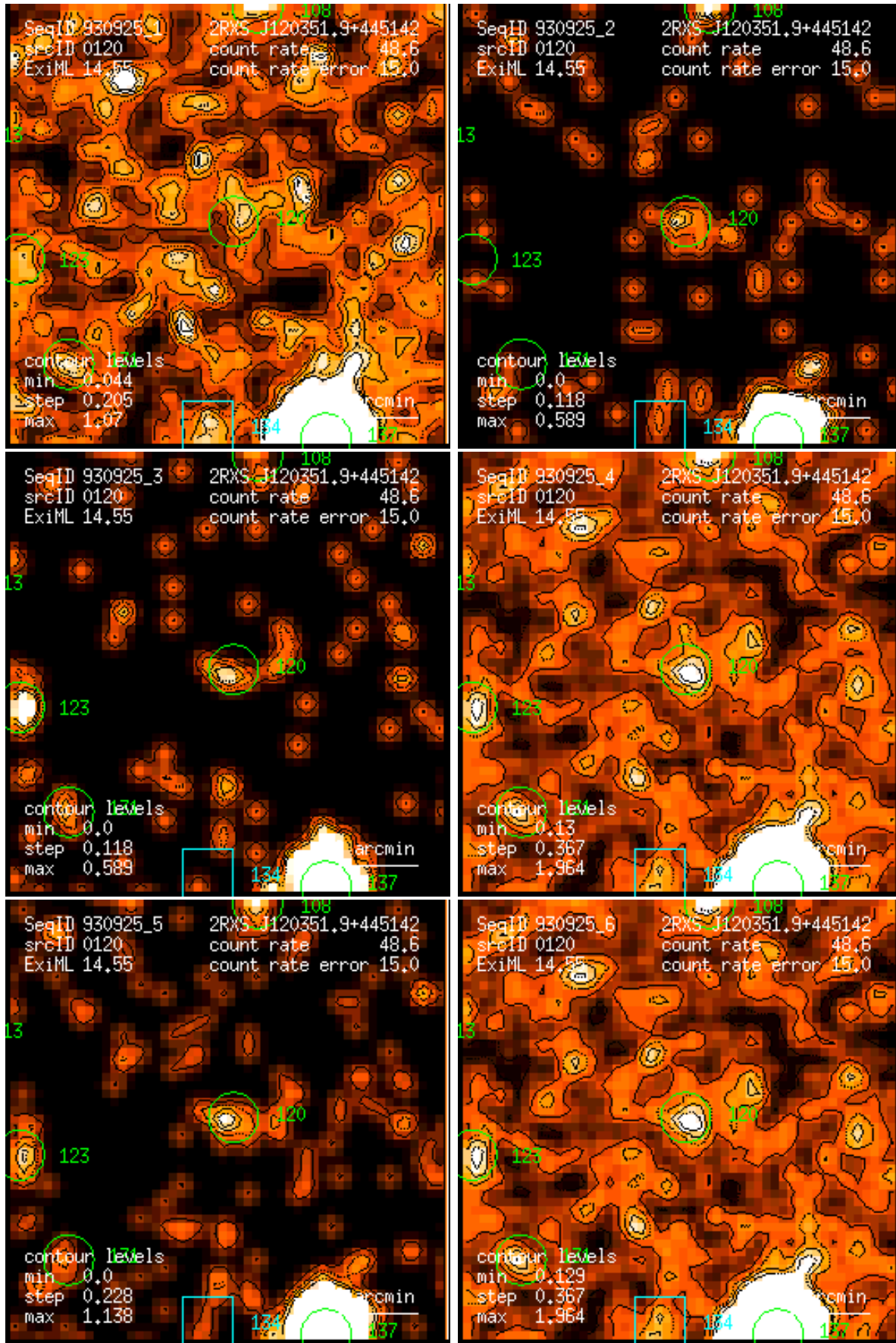
Figure 120: RASS 930925: detection 0120: band rate images, Gaussian filter: (1) PSPC channels 11 – 41, (2) 52 – 90, (3) 91 – 201, (4) 11 – 235, (5) 52 – 201, (6) 11 – 201. Broad band rates in counts/ks. Band rate contour levels in counts/ks/arcmin 2 .
