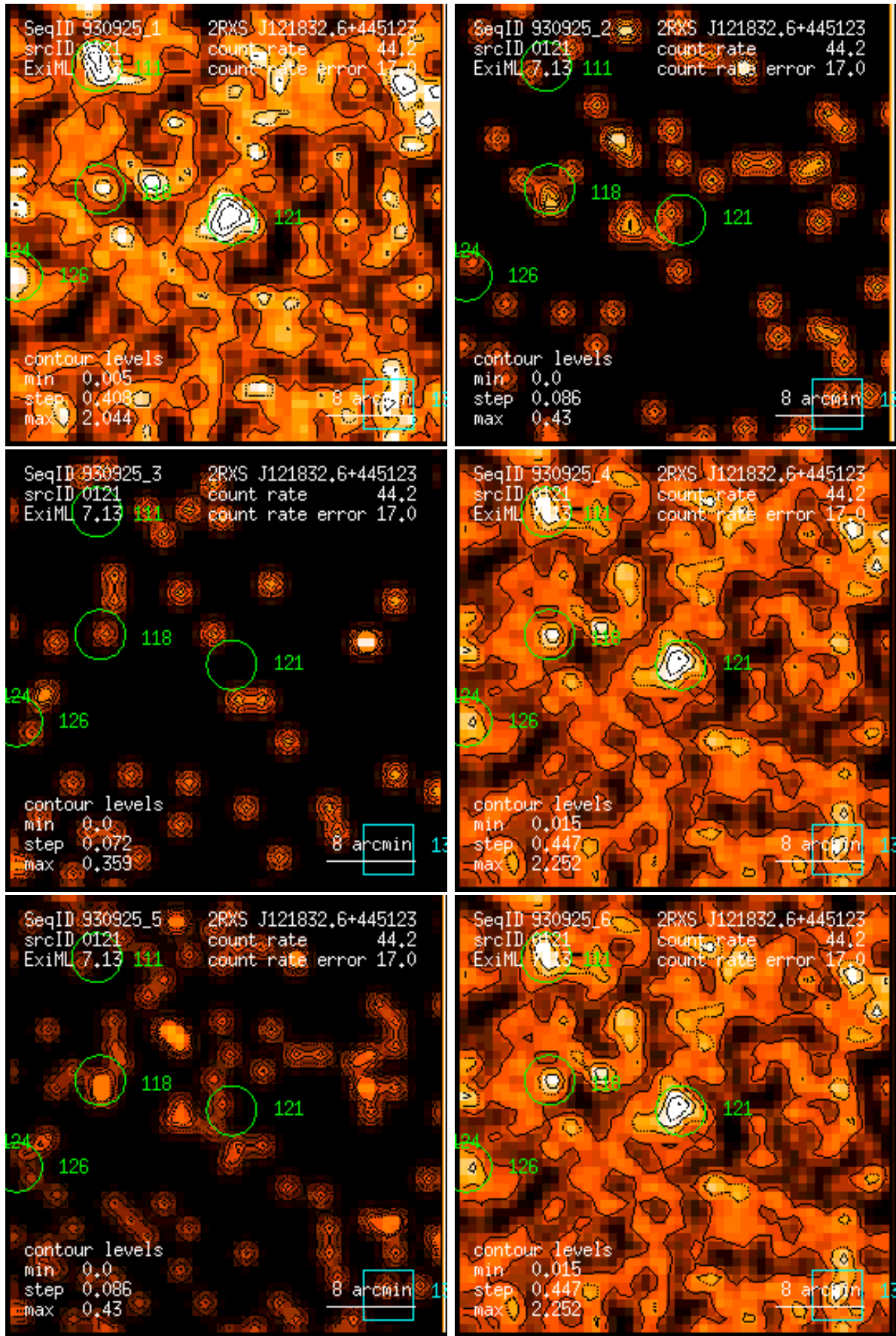
Figure 121: RASS 930925: detection 0121: band rate images, Gaussian filter: (1) PSPC channels 11 – 41, (2) 52 – 90, (3) 91 – 201, (4) 11 – 235, (5) 52 – 201, (6) 11 – 201. Broad band rates in counts/ks. Band rate contour levels in counts/ks/arcmin 2 .
