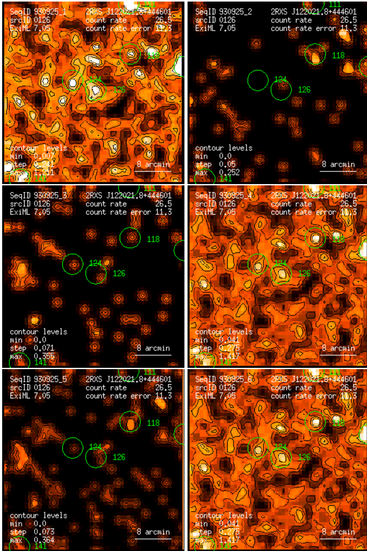
Figure 126: RASS 930925: detection 0126: band rate images, Gaussian filter: (1) PSPC channels 11 – 41, (2) 52 – 90, (3) 91 – 201, (4) 11 – 235, (5) 52 – 201, (6) 11 – 201. Broad band rates in counts/ks. Band rate contour levels in counts/ks/arcmin 2 .
