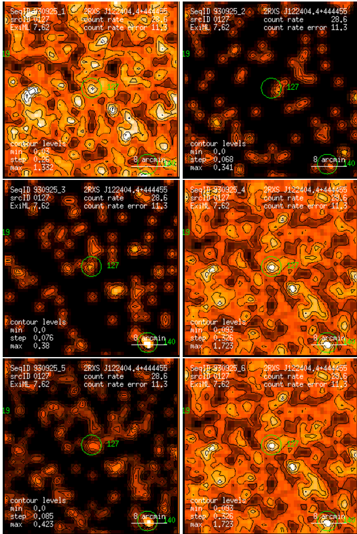
Figure 127: RASS 930925: detection 0127: band rate images, Gaussian filter: (1) PSPC channels 11 – 41, (2) 52 – 90, (3) 91 – 201, (4) 11 – 235, (5) 52 – 201, (6) 11 – 201. Broad band rates in counts/ks. Band rate contour levels in counts/ks/arcmin 2 .
