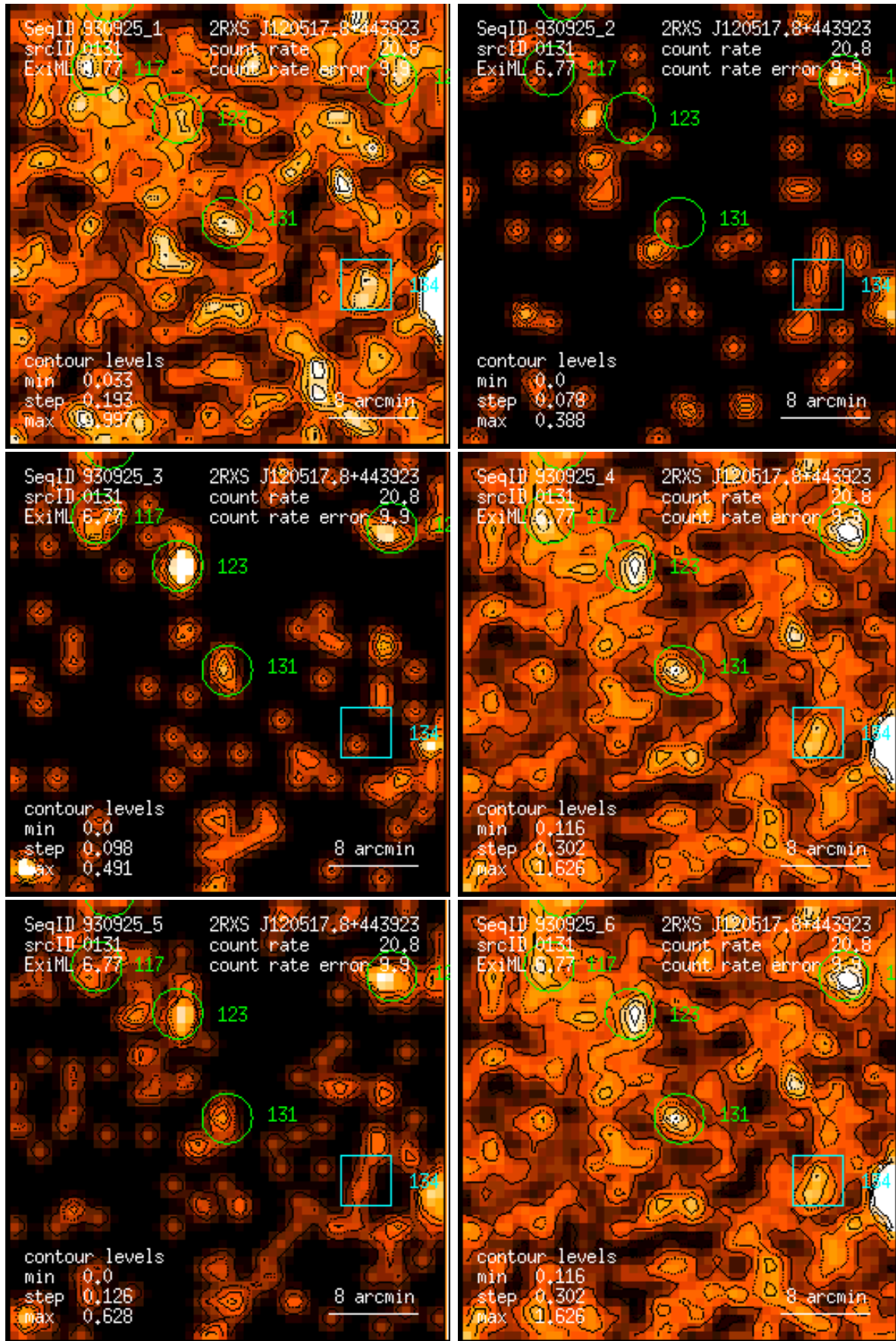
Figure 131: RASS 930925: detection 0131: band rate images, Gaussian filter: (1) PSPC channels 11 – 41, (2) 52 – 90, (3) 91 – 201, (4) 11 – 235, (5) 52 – 201, (6) 11 – 201. Broad band rates in counts/ks. Band rate contour levels in counts/ks/arcmin 2 .
