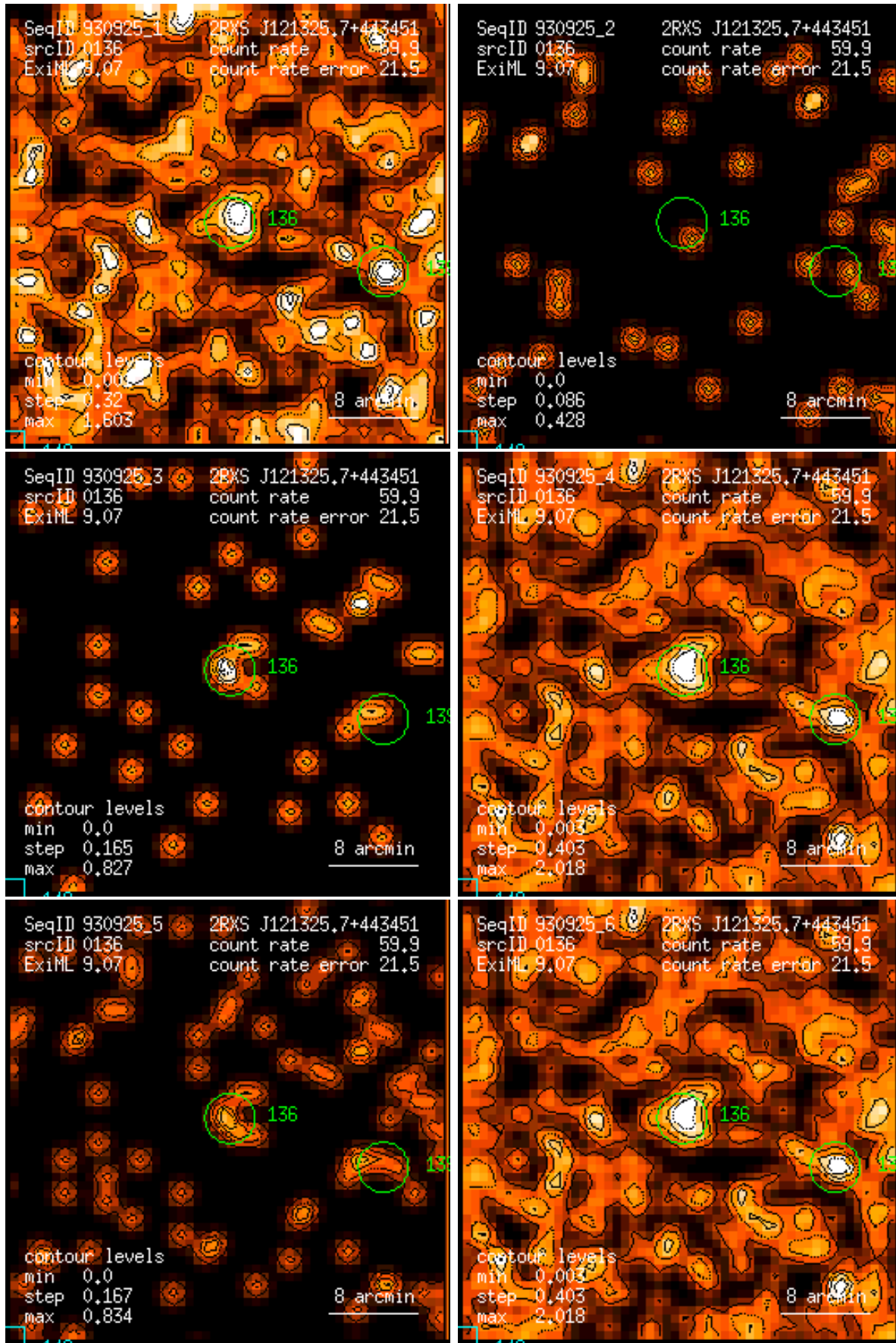
Figure 136: RASS 930925: detection 0136: band rate images, Gaussian filter: (1) PSPC channels 11 – 41, (2) 52 – 90, (3) 91 – 201, (4) 11 – 235, (5) 52 – 201, (6) 11 – 201. Broad band rates in counts/ks. Band rate contour levels in counts/ks/arcmin 2 .
