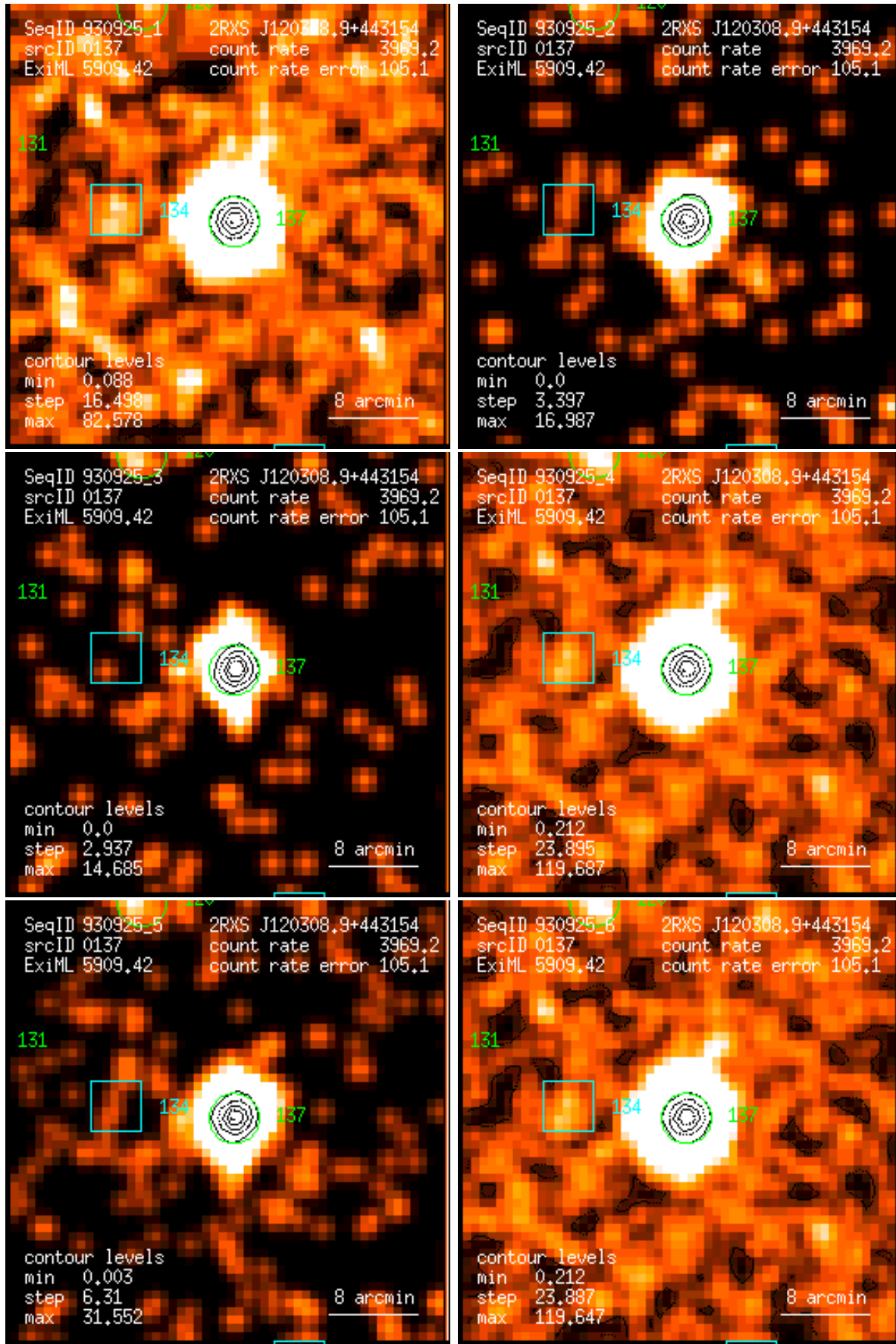
Figure 137: RASS 930925: detection 0137: band rate images, Gaussian filter: (1) PSPC channels 11 – 41, (2) 52 – 90, (3) 91 – 201, (4) 11 – 235, (5) 52 – 201, (6) 11 – 201. Broad band rates in counts/ks. Band rate contour levels in counts/ks/arcmin 2 .
