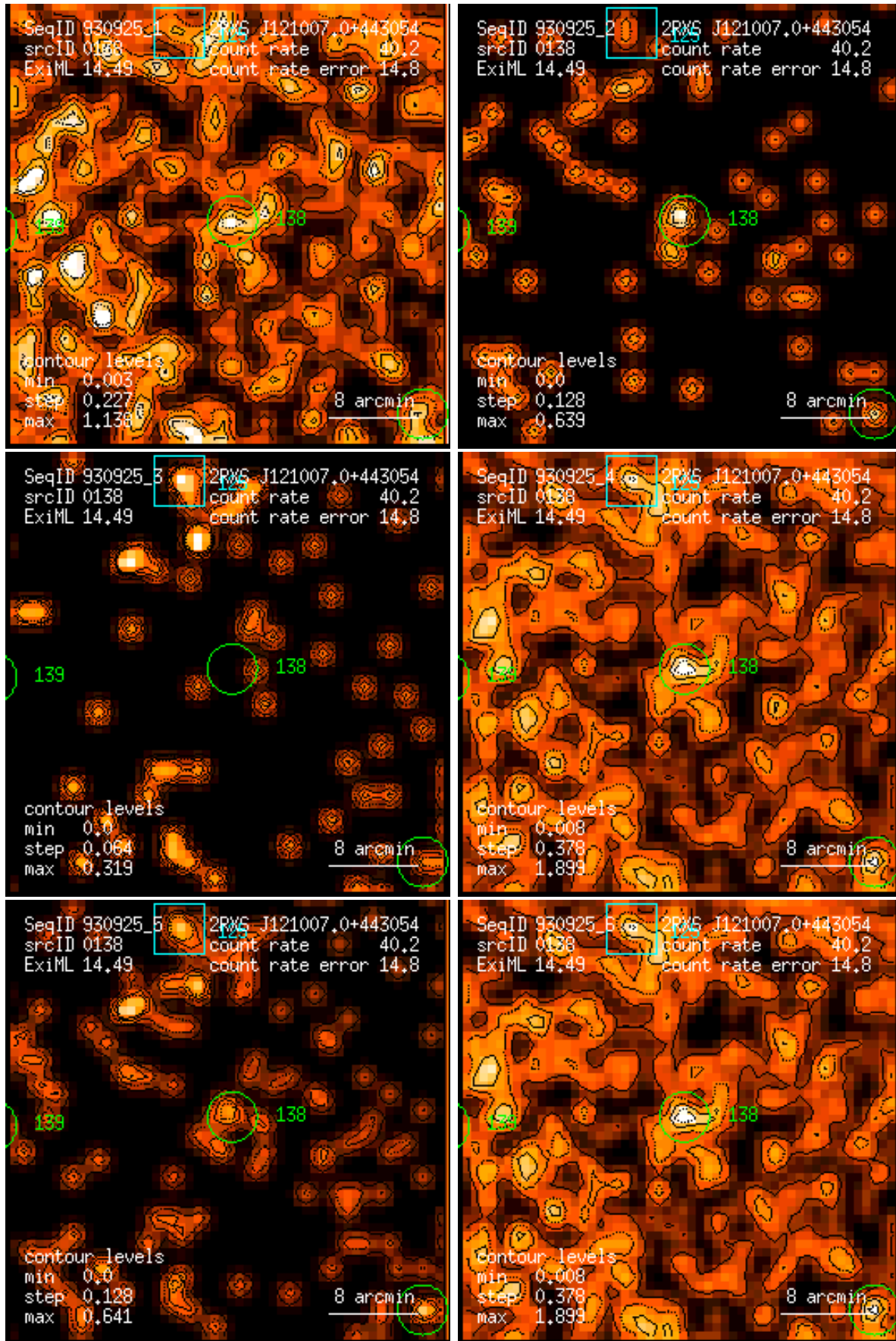
Figure 138: RASS 930925: detection 0138: band rate images, Gaussian filter: (1) PSPC channels 11 – 41, (2) 52 – 90, (3) 91 – 201, (4) 11 – 235, (5) 52 – 201, (6) 11 – 201. Broad band rates in counts/ks. Band rate contour levels in counts/ks/arcmin 2 .
